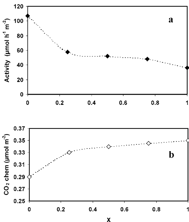
Fig. 1. Acidic and basic properties of the Mg x Ni 1-x Al 2 O 3 spinel oxides supported on γ-alumina (first series): (a) activity in the DM33B1 isomerization at 300 °C; (b) CO 2 chemisorption at 25 °C.
