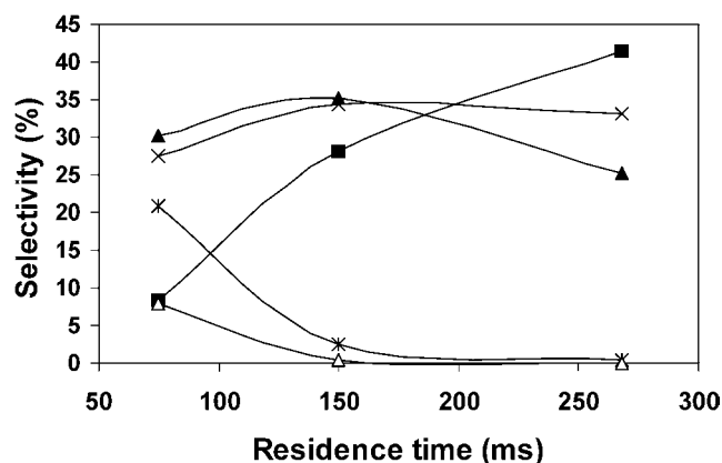
Fig. 3. Influence of the residence time on the C-products distribution upon reaction at T = 700 °C, P = 11 bar and water:ethanol molar ratio = 4: (■) CO 2 , (▲) CO, (x) CH 4 , (*) C 2 H 4 + C 2 H 6 , (Δ) CH 3 CHO.
