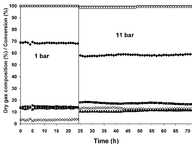
Fig. 2. Stability test over N-Rh/1-Mg 1 Al at P = 1 and 11 bar, T = 700 °C, GHSV = 13,400 h -1 and water:ethanol molar ratio R = 4 : (O) ethanol conversion; (◆) H 2 ; (■) CO 2 ; (▲) CO; (◇) CH 4 . Other gases (acetaldehyde + ethylene + ethane) <1%.
