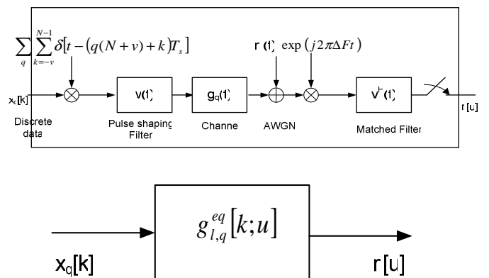
Figure 16: Equivalent channel transfer function with synchronization errors
