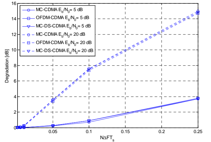
Figure 4: comparison between degradation of different spreading schemes
