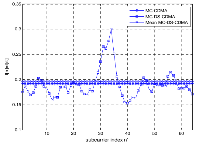
Figure 14: Interference power (MMSE and BranA channel) k_0 = -5 samples.
