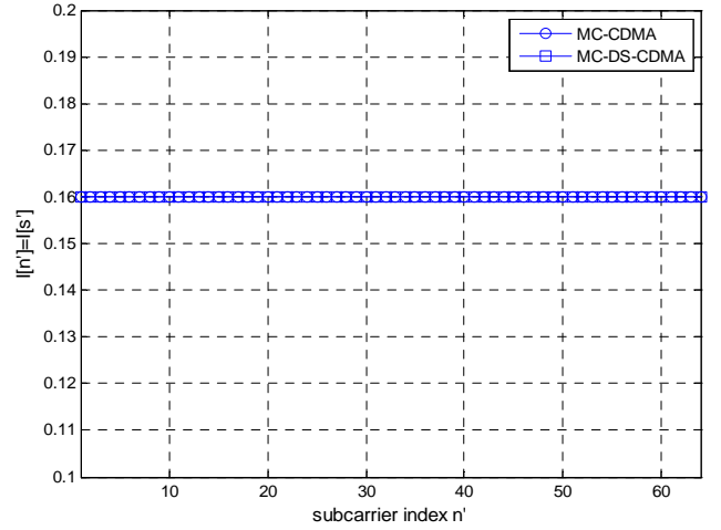
Figure 13: Interference power (MMSE and Gaussian channel) k_0 = -5 samples.
