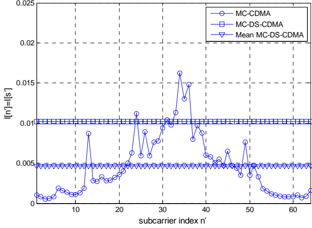
Figure 11: Mean Interference power (MMSE and BRAN A channel) \Delta T/T_s = 390 ppm
