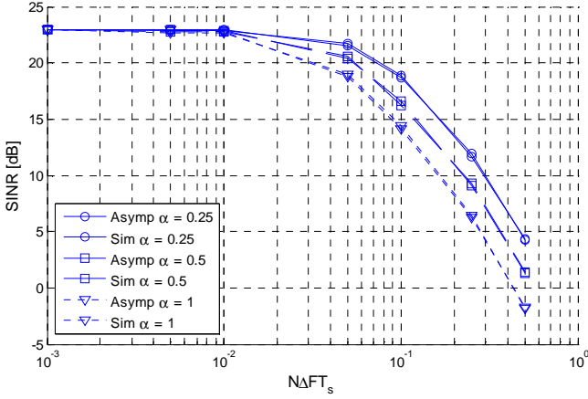
Figure 5: sensitivity of MC-DS-CDMA to system load (Gaussian channel).
