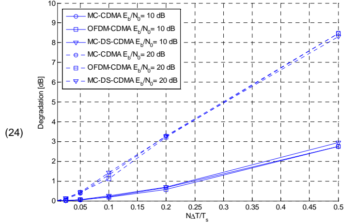
Figure 9: comparison between degradation of different spreading schemes (BRAN A channel, full load).
