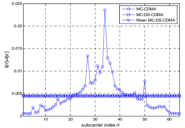
Figure 10: Mean Interference power (ZF and BRAN A channel) \Delta T/T_s = 390 ppm.
