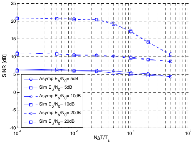
Figure 8: validation of theoretical model (BRAN A channel).
