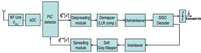
Figure 17: Iterative receiver scheme.
