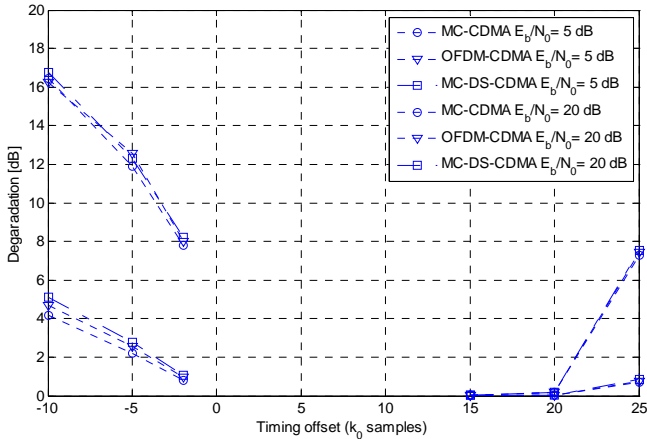
Figure 15: comparison between degradation of different spreading schemes (BranA channel, full load).
