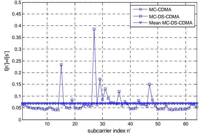
Figure 6: Mean Interference power (ZF and BRAN A channel).
