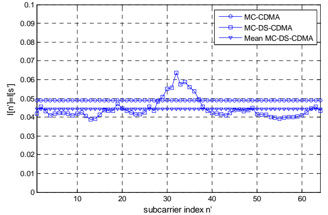
Figure 7: Mean Interference power (MMSE and BRAN A channel).
