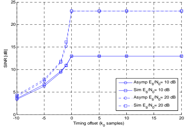
Figure 12: validation of theoretical model (Gaussian channel).
