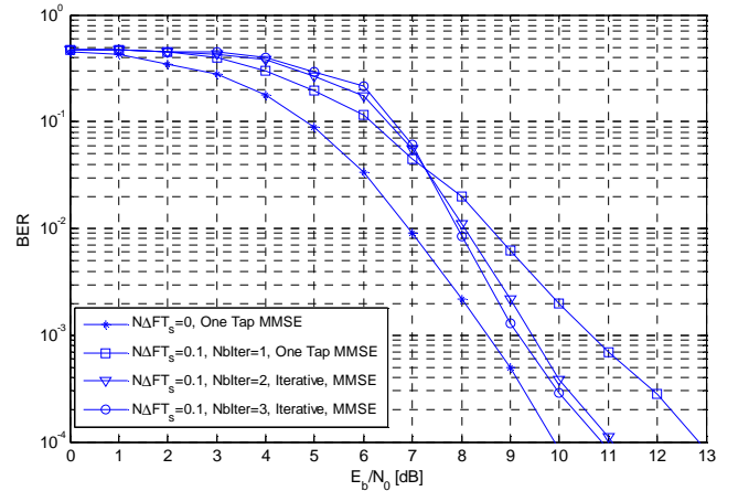
Figure 18: BER performance of iterative receiver in OFDM-CDMA system, BranA channel, 16-QAM constellation.
