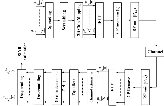
Figure 1- OFDM-CDMA Transceiver.
