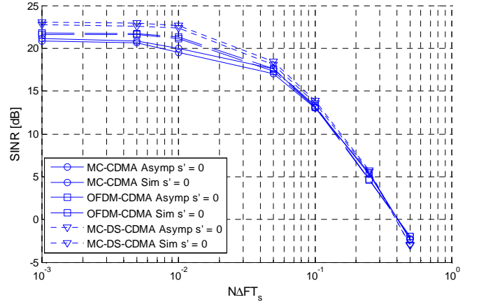
Figure 3: validation of theoretical model (BRAN A).
