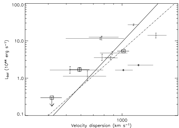
Figure 19. Bolometric X-ray luminosity versus optical velocity dispersion for the Cl1216–1201, Cl1054–1145, and Cl1040–1155 clusters. The symbols are as described in Fig. 18. The Cl1040–1155 point is a 3\sigma detection limit based on the background level within a radius of 90 arcsec. The solid line shows the best-fitting relation of Xue & Wu (2000), whereas the dotted line shows that of Mahdavi & Geller (2001). In addition to the optically selected clusters of Lubin et al. (2004), RX J1716.6+6708 (Gioia et al. 1999, z = 0.81 ) also appears significantly underluminous in X-rays for its velocity dispersion.
