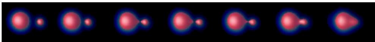
Figure 9: Same as figure 8 for center of mass energy 74.45 MeV (just above fusion barrier).
