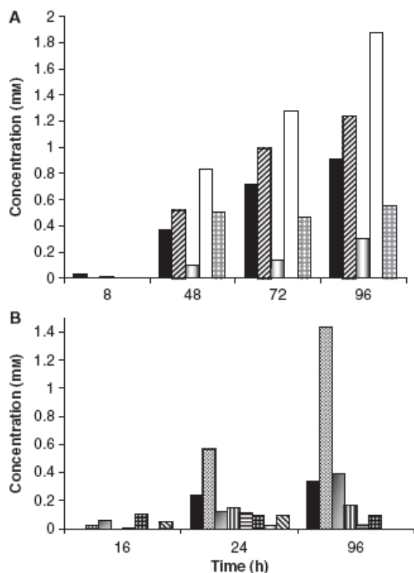
Fig. 5. Time dependence of concentration of metabolites released during the growth of R. albus 20 on Sigmacell 20 cellulose (A) or wheat straw (B). Values were determined from the signal intensities in the 1 H NMR spectra. At least two signal integrations were carried out. Standard deviations were usually less than 15%. □ Ara; ▨ \alpha Ara Xyl ; ▩ \alpha and \beta CB red or \alpha and \beta cellodextrins (CD red ); ▪ CD int ; ■ \alpha Galf Man ; ● \alpha and \beta Glc; ▤ Glc-IP; ▥ Glc Xyl ; □ X2; ▧ Xyl; ▨ Xyl int .
