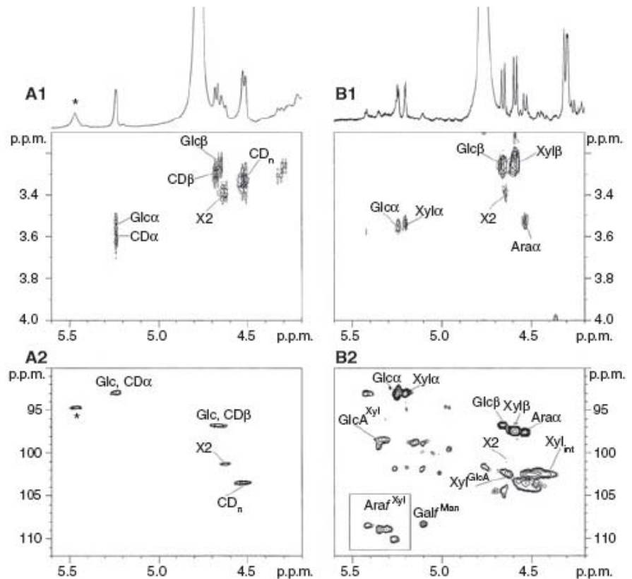
Fig. 4. Spectra of culture medium of R. albus 20 grown with cellulose (A) or wheat straw (B) after 4 days. (A1, B1) Anomeric part of COSY spectrum. (A2, B2) Anomeric part of HSQC spectrum. Ara, arabinose; Ara Xyl , \alpha -arabinofuranose linked to O2, O3 or O2,O3 of xylose; CD \alpha\beta , \alpha - and \beta -glucose units of reducing end of cellobiose; CD n , nonreducing end glucose of cellobiose or terminal and internal units of celloextrins; Galf Man , \alpha -galactofuranose of galactomannans; Glc, glucose; GlcA Xyl , \alpha -glucuronic acid linked to O2 of xylose unit; X2, unknown derivative of glucose; Xyl, xylose; Xyl GlcA , xylose unit substituted at O2 by \alpha -GlcA; Xyl int , internal units of nonsubstituted xylooligosaccharides; *, glucose 1-phosphate derivative.
