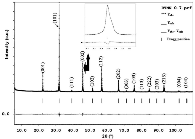
FIG. 1. XRD patterns for a cubic ceramic sample of \text{Ba}_{1-x}\text{Na}_x\text{Ti}_{1-x}\text{Nb}_x\text{O}_3 with x=0.70 .
