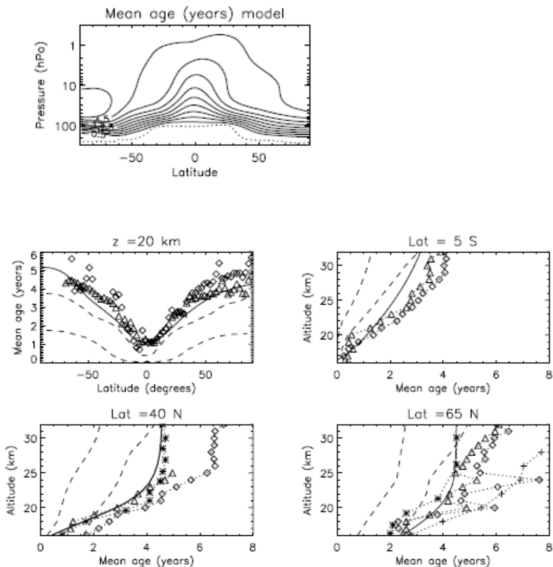
Fig. 4. Annually and zonally averaged mean age of air relative to the equatorial tropopause and after 20-years of the LMDz-REPROBUS simulation (see text for details). (a) Latitude-altitude section, the dotted thick line indicates the thermal tropopause and the contour interval is 0.5 year.; (b) Latitudinal variation at the altitude z=20 km. (c) vertical profile at the latitude 5 S, (d) vertical profile at the latitude 40 N, and (e) vertical profile at the latitude 65 N. In (b), (c), (d), and (e) the solid line is for the model values while the various symbols are derived from observations: in situ \text{CO}_2 (triangles) are from Boering et al. (1996) and Andrews et al. (2001b), in situ \text{SF}_6 (diamonds) are from Elkins et al. (1999), Ray et al. (1999) and \text{SF}_6 whole-air samples are from Harnish et al. (1996) (asterisk outside the vortex and crosses inside the vortex). See also Hall et al. (1999) for details on those measurements. The dashed lines represent the range of most models involved in the Models and Measurements II project (Hall et al., 1999).
