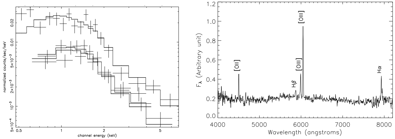
Fig. 8. MOS1 MOS2 (the two lower functions) and pn (upper one) X-ray spectra of a source which is only showing mild X-ray absorption with N_{\text{H}}^{\text{int}}=2.5 \cdot 10^{21} \text{ cm}^{-2} . The crosses represent the data points and the solid lines represent the folded model simultaneously fitted to the data of the 3 detectors (left). The optical counterpart has been identified as a Seyfert 2 lying at a redshift z = 0.207 . We clearly observe the [OIII] lines around 6000 \text{ \AA} (right). This is source #53 in Table 4.
