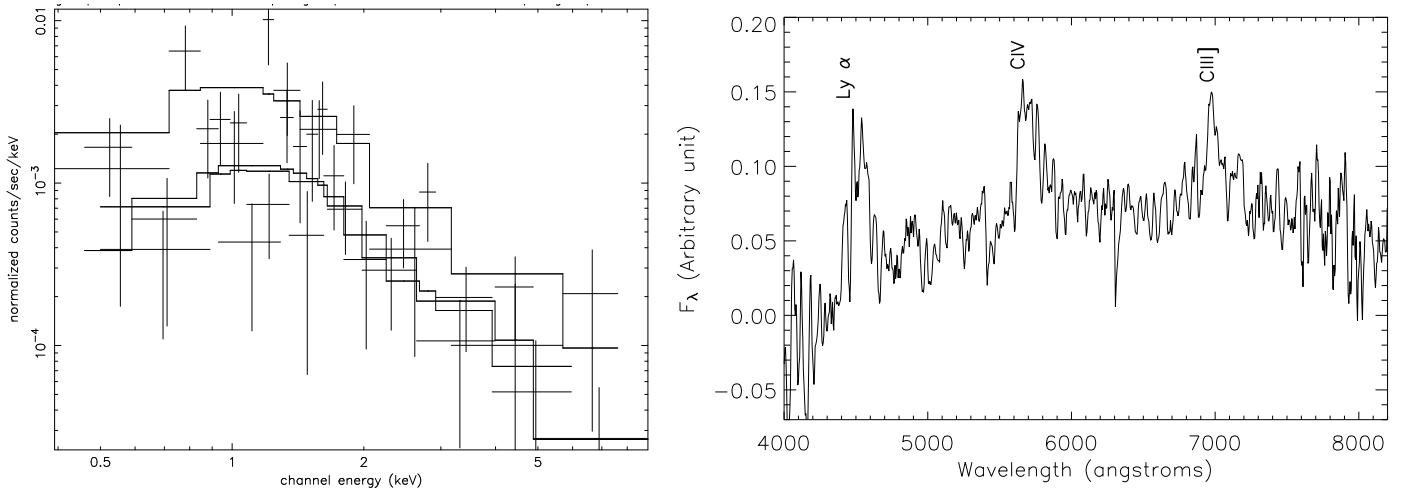
Fig. 15. MOS1 MOS2 (the two lower functions) and pn (upper one) X-ray spectra of a source which is showing strong X-ray absorption with N_{\text{H}}^{\text{int}} = 4 \cdot 10^{22} \text{ cm}^{-2} . The crosses represent the data points and the solid line represent the folded model simultaneously fitted to the data of the 3 detectors (left). The optical counterpart has been identified as a BLAGN lying at a redshift z = 2.66 (right). This is source #20 in Table 4.
