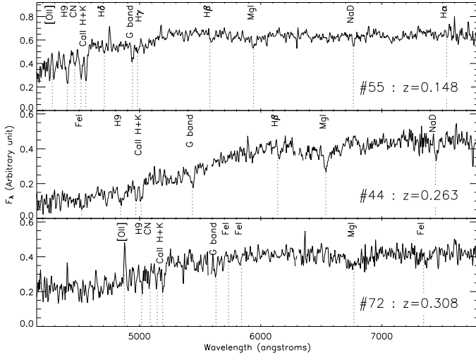
Fig. 16. The 3 XBONG candidates. Each of these 3 XBONG lacks emission lines, except for [OII] in source #72. This source presents strong absorption in the X-rays ( N_{\text{H}}^{\text{int}}=3.86 \times 10^{22} \text{ cm}^{-2} ).
