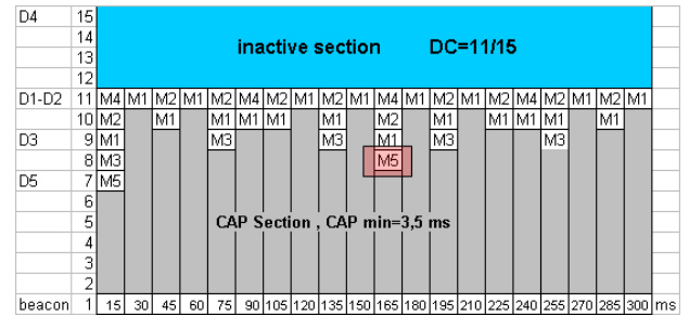
Figure 6. Arbitration table scheduling with DC = 0.73
