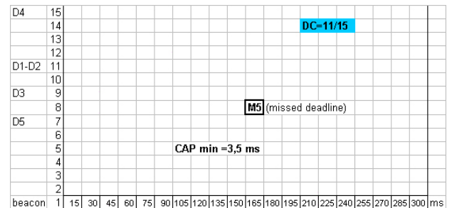
Figure 7. Sort of the missed deadline on a given scenario
