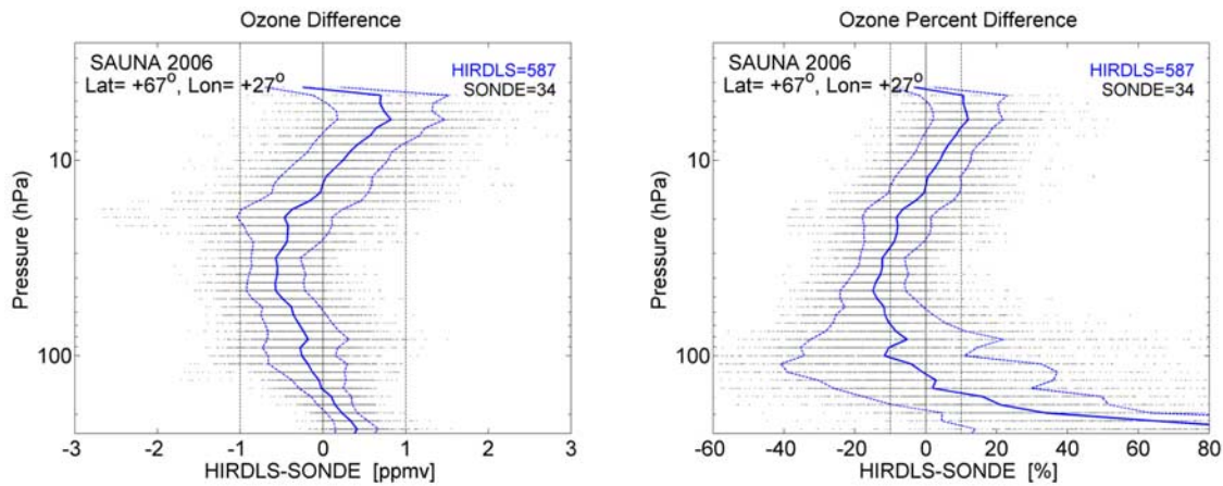
Figure 3. Shown are mean (solid blue) and the standard deviation (dashed blue) of the ozone differences between HIRDLS and ozonesondes (34 sondes using 0.5% KI cathode solution) from the spring 2006 Sodankylä Total Ozone Intercomparison and Validation (SAUNA) campaign carried out at Sodankylä, Finland (67°N, 27°E).
