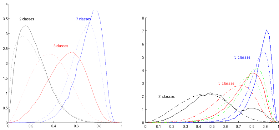
Figure 1: Density of conflict for (left) two uniform random experts and (right) three uniform random experts; with and without decision change
