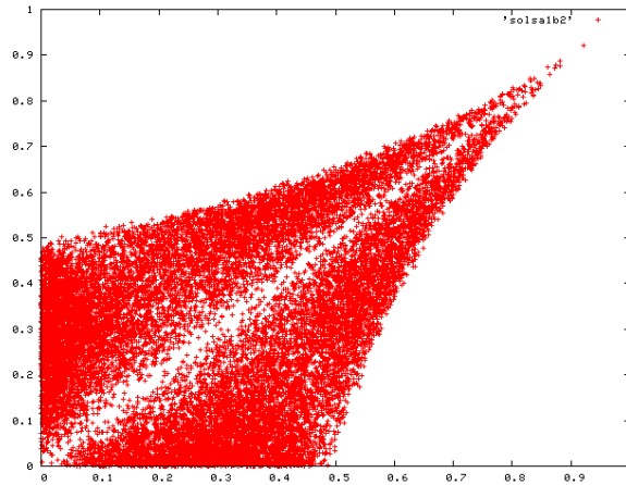
Figure 3: Decision changes, projected on the plane a_1, b_2 .
