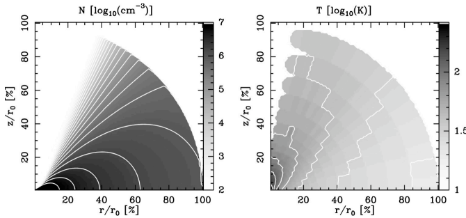
Fig. 6. Density and temperature distributions for the 2D model presented in a logarithmic grey scale, with 20 logarithmic levels from 10^2 to 10^7 \text{ cm}^{-3} for density and 10 logarithmic levels from 10 K to 263 K.
