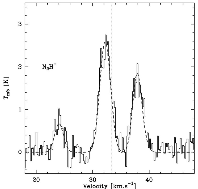
Fig. 8. Emission of N 2 H + from MM1 object overlaid by 1D model of the source (dashed line). The triplet shape is completely reproduced using our RATRAN molecular datafile. Spectra velocity resolutions are kept identical to observational resolutions reported in Table 2.
