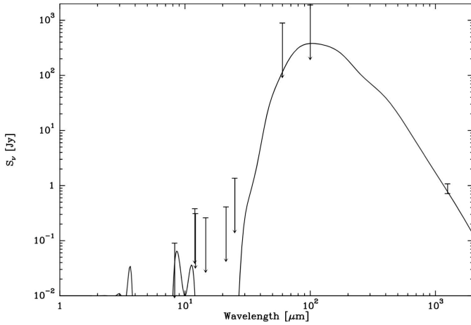
Fig. 11. Spectral energy distribution of MM2 overlaid with the 1D model result. Infrared emission has always an upper limit due to the non-detection of the source.
