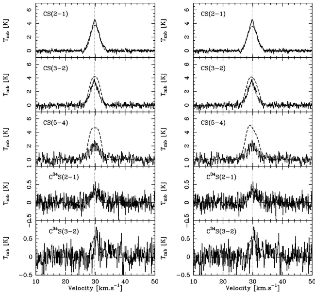
Fig. 12. Emission of CS from MM2 object overlaid by 1D static (left) and 1D with infall ( v_{in} = -1.0 \text{ km.s}^{-1} ) model of the source (dashed lines). Spectra velocity resolutions are kept identical to observational resolutions reported in Table 2.
