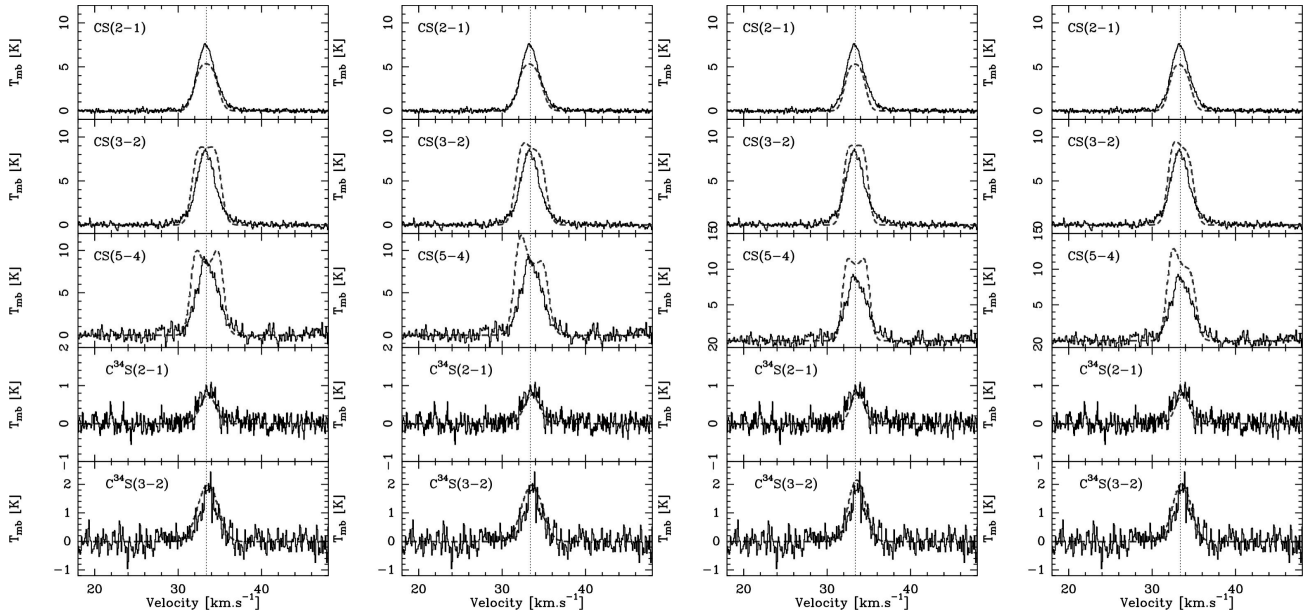
Fig. 7. Emission of CS and C^{34}S from MM1 object (continuous line) overlaid by –from left to right– 1D static, 1D with infall ( v_{in} = -0.4 \text{ km}\cdot\text{s}^{-1} ), 2D static and 2D with infall ( v_{in} = -0.4 \text{ km}\cdot\text{s}^{-1} ) model line emissions (dashed). Spectra velocity resolutions are kept identical to observational resolutions reported in Table 2.
