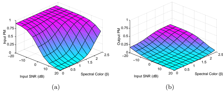
Figure 4. Periodicity measures (PM) achieved on simulated data in different input SNRs and different spectral colors, (a) before and (b) after denoising. The decrease of PM is used as a necessary, but not sufficient, measure of the filtering performance.
