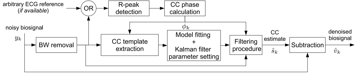
Figure 1. The overall denoising scheme. As shown in this figure the R-peaks of the contaminating signals (CC) may either be detected from an arbitrary reference ECG or from the noisy biosignal after baseline wander (BW) removal.
