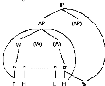
Figure 1. The intonational structure of the Korean language as described in the K-ToBI framework.
