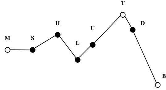
Figure 3. INTSINT, a system for annotation of intonation.
