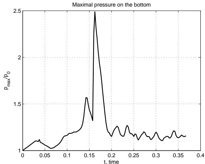
Fig. 19. Water drop test case. Maximum bottom pressure as a function of time. view, is an immediate byproduct of our cell-centered finite volume method.
