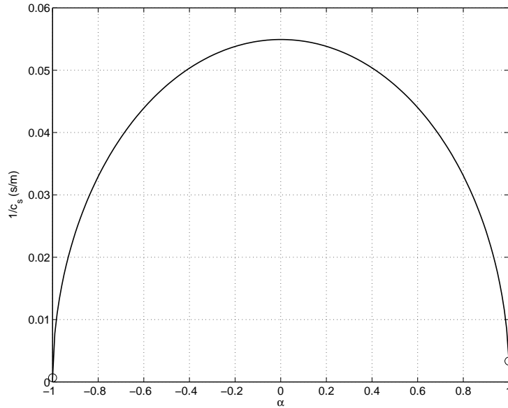
Fig. 1. Speed of sound c_s as a function of \alpha . In order to make the curve more visible, the inverse of the speed of sound 1/c_s is plotted. The end points, represented by circles, correspond to pure liquid (left) and pure gas (right).
