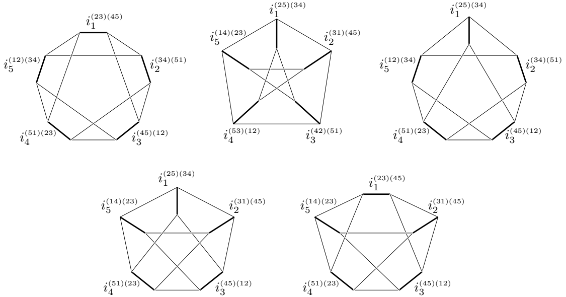
Figure 1: The five classes of pairings: from the upper left: (10), (5,5), (7,3), (6,4) and (4,3,3).
