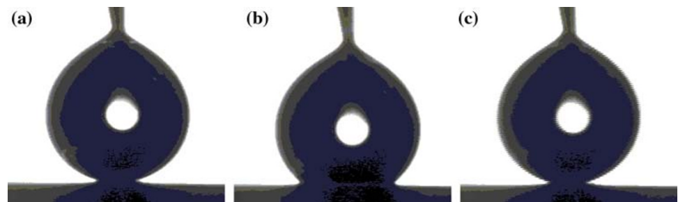
Fig. 31 Reversible EWOD observed on a drop deposited on a superhydrophobic silicon nanowires surface. (a) No tension applied, (b) a 150 V rms tension applied ( f = 1 kHz), (c) the tension is cut, the drop returns to its initial state
