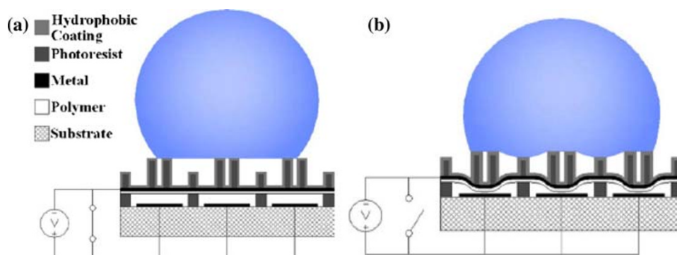
Fig. 13 The operation concept of SWIM: (a) at initial state, the droplet merely contacts the higher posts and (b) at actuated state, the droplet will contact with both the higher and lower posts. Reprinted with permission from [39]. Copyright 2007 Institute of Physics
