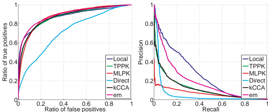
Figure 5: Performance of different methods for the reconstruction of the PPI network (from [8]): ROC (left) and precision/recall (right) curves.
