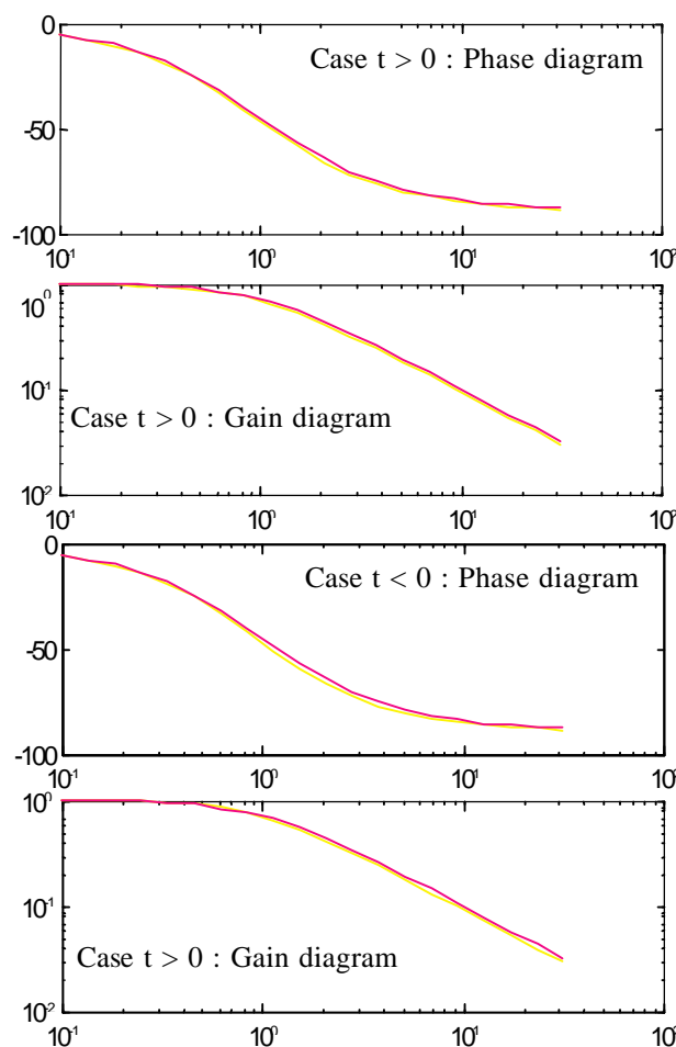
Figure 4. Bode plots
