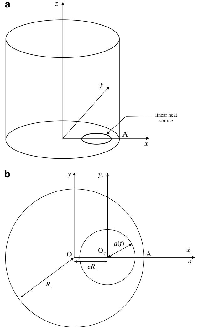
Fig. 9. Geometry of the thermal problem: (a) tridimensional visualization and (b) geometry of the circular crack.
