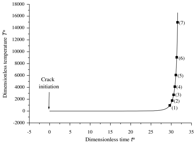
Fig. 11. Numerical simulation of the temperature evolution at point A on the specimen surface ( a_0 = 10 \mu\text{m} , e = 0.5 ).
