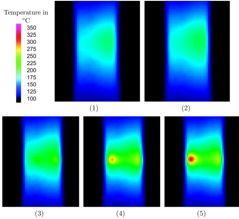
Fig. 4. Temperature fields on the specimen surface just before fracture ( \Delta\sigma = 335 MPa, N_F = 8.37 \times 10^7 cycles). (1) N = 8.35890 \times 10^7 cycles, (2) N = 8.36500 \times 10^7 cycles, (3) N = 8.36968 \times 10^7 cycles, (4) N = 8.36996 \times 10^7 cycles, and (5) N = 8.37000 \times 10^7 cycles.
