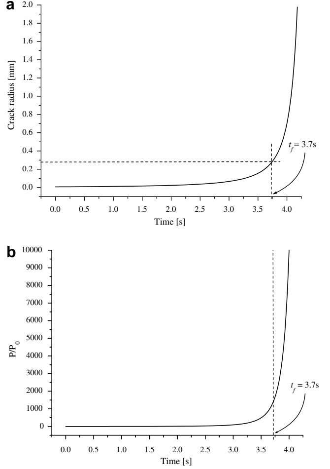
Fig. 8. Model of the crack propagation: (a) evolution of the crack radius and (b) evolution of the dissipated power per unit length of crack.
