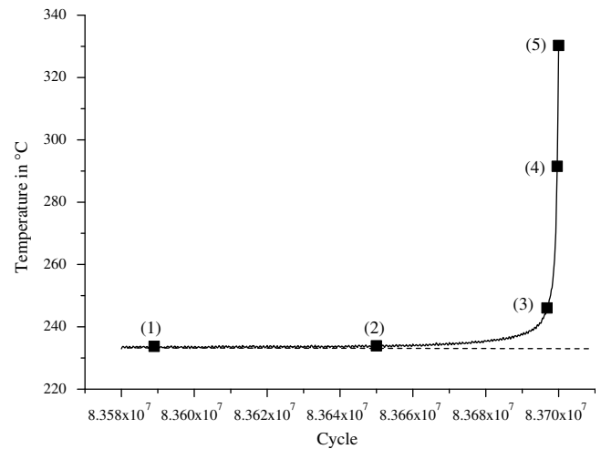
Fig. 3. Temperature evolution on the specimen surface just before fracture ( \Delta\sigma = 335 \text{ MPa} ; N_F = 8.37 \times 10^7 cycles).
