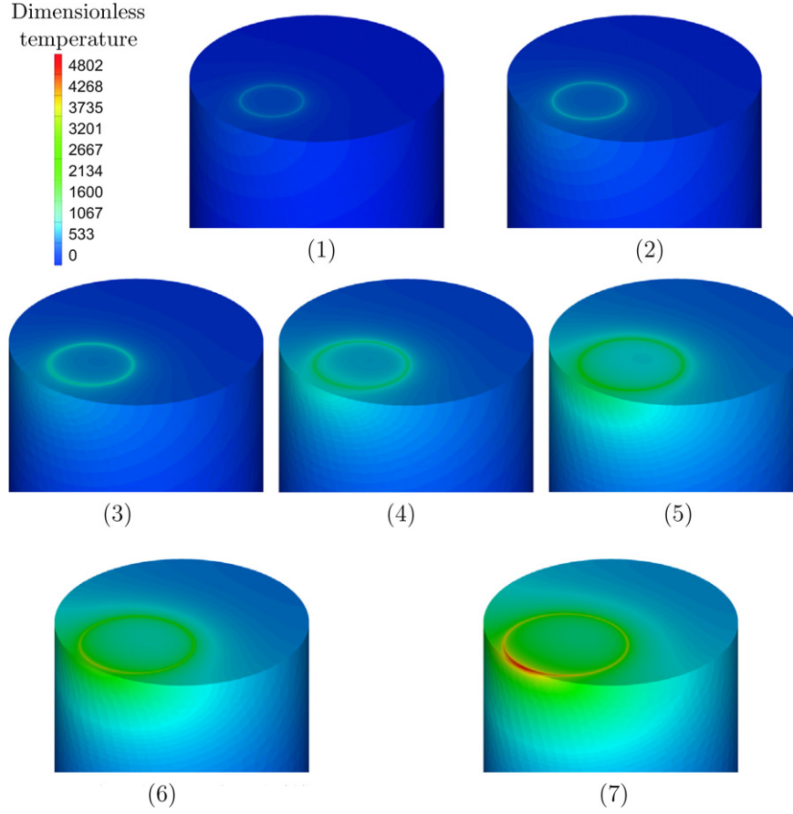
Fig. 10. Numerical simulation of the temperature field in the specimen for various times before fracture ( a_0 = 10 \mu\text{m} , e = 0.5 ). (1) t^* = 29.65 ; a^* = 0.227 , (2) t^* = 30.23 ; a^* = 0.277 , (3) t^* = 30.59 ; a^* = 0.317 , (4) t^* = 30.89 ; a^* = 0.357 , (5) t^* = 31.15 ; a^* = 0.397 , (6) t^* = 31.36 ; a^* = 0.437 , and (7) t^* = 31.55 ; a^* = 0.477 .
