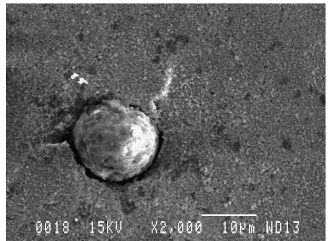
Fig. 6. Observation by scanning electron microscopy of the inclusion in the center of the fatigue crack.
