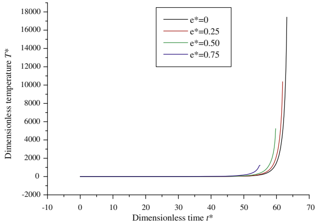
Fig. 13. Effect of eccentricity on the temperature evolution ( a_0 = 20 \mu\text{m} ).
