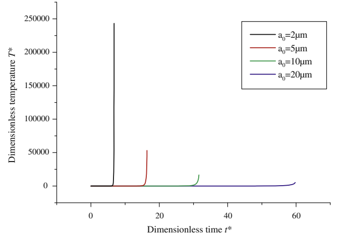
Fig. 12. Effect of the initial radius of the crack on the temperature evolution ( e = 0.5 ).
