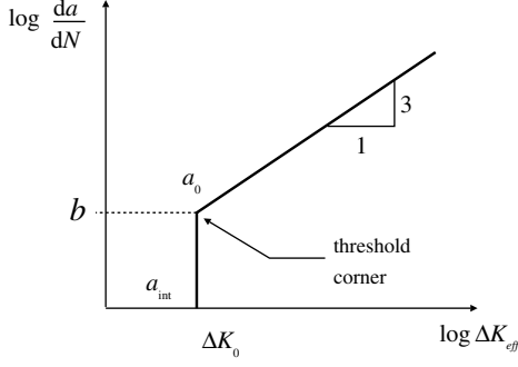
Fig. 7. Crack growth rate according to the stress intensity factor.
