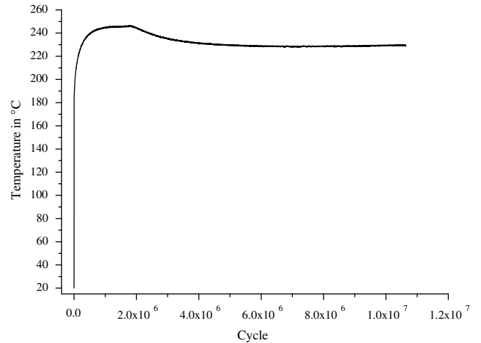
Fig. 2. Temperature evolution on the specimen surface during ultrasonic fatigue test without fracture ( \Delta\sigma = 315 \text{ MPa} ).
