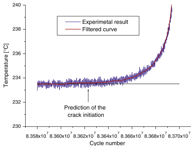
Fig. 15. Experimental determination of crack initiation.
