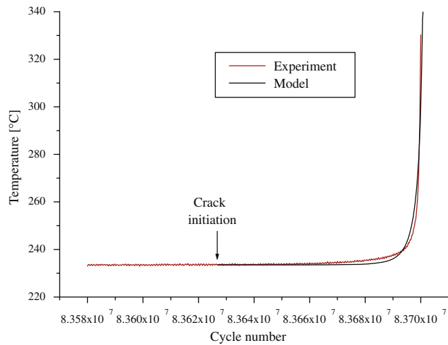
Fig. 14. Comparison between model and experiment.
