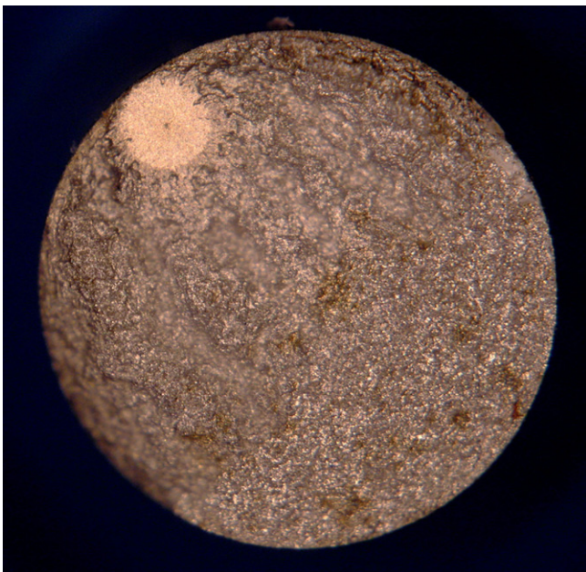
Fig. 5. Postmortem observation by optical microscopy of the fracture surface: propagation of a fish eye fatigue crack.
