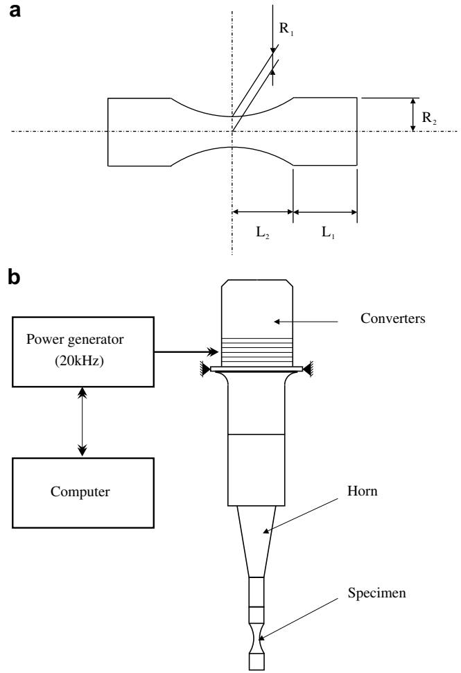
Fig. 1. Ultrasonic fatigue test: (a) geometry of the specimen and (b) ultrasonic fatigue machine.
