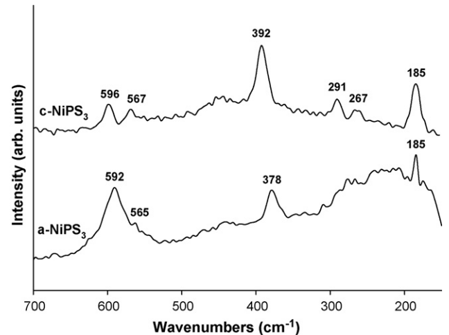
Fig. 2. Raman spectra of the well-crystallized c-NiPS 3 and a-NiPS 3 synthesized at low temperature.
