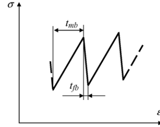
Fig. 8. Middle-band time and formation-band time in a scheme stress strain curve.
