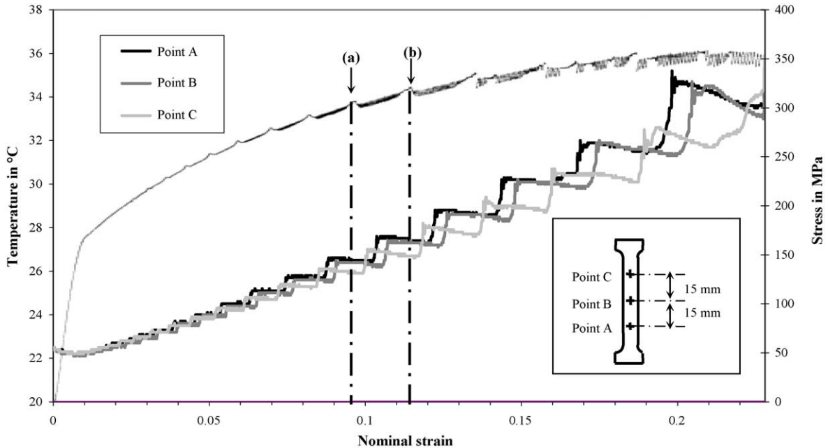
Fig. 1. Stress–strain curve and temperature evolution.
