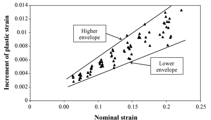
Fig. 9. Increment of plastic strain vs. nominal strain.
