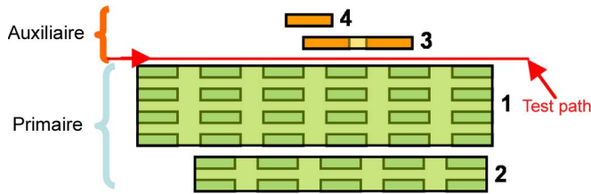
Fig. 16. Homogenization of rectangular wires.
