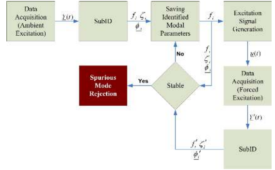
Fig. 1. Online Modal Parameter Estimation using Output-only Subspace Identification.
