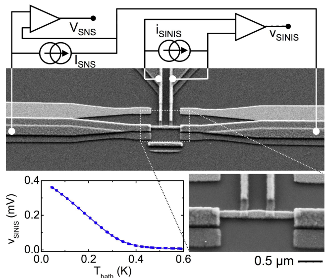
FIG. 1: (Color online) Top: SEM image of sample 2 containing a S-N-S junction of 1.5 \mu\text{m} length with a sketch of the measurement circuit. Two tunnel probes (top of the image) are connected to the normal metal embedded between two superconducting banks (on left and right sides of the image). The overlap of the superconducting banks (dark grey) with the normal metal layer (light grey) is visible. During the measurement, the S-I-N-I-S junction is biased at a fixed current I_{SINIS} and the voltage drop V_{SINIS} is monitored. Bottom: Temperature dependence of the voltage V_{SINIS} of the same sample with a current bias I_{SINIS} = 6 \text{ pA} (no current is flowing through the S-N-S junction) and zoom of the sample image.
