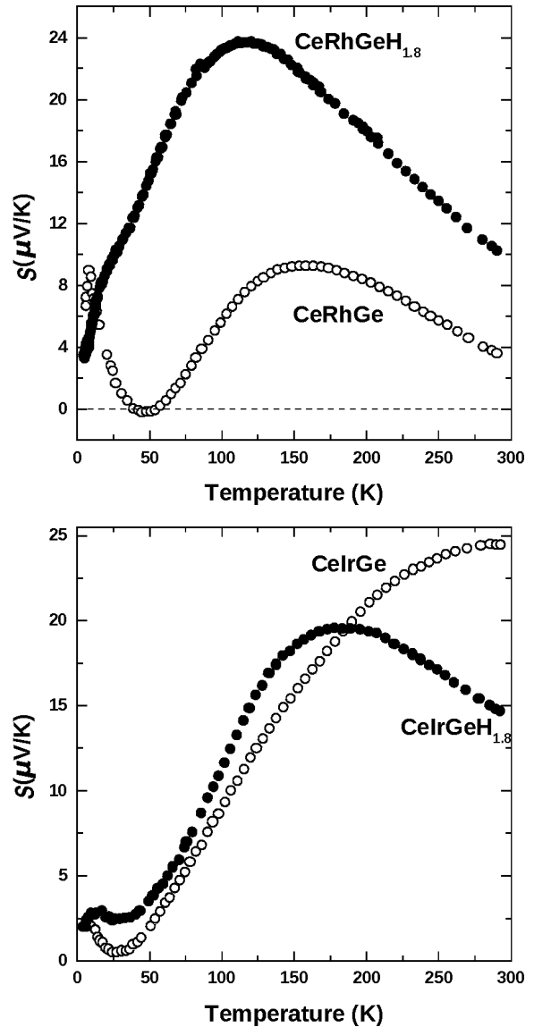
Fig. 7. Temperature dependence of the thermoelectric power S for \text{CeRhGe} , \text{CeIrGe} and their hydrides.
