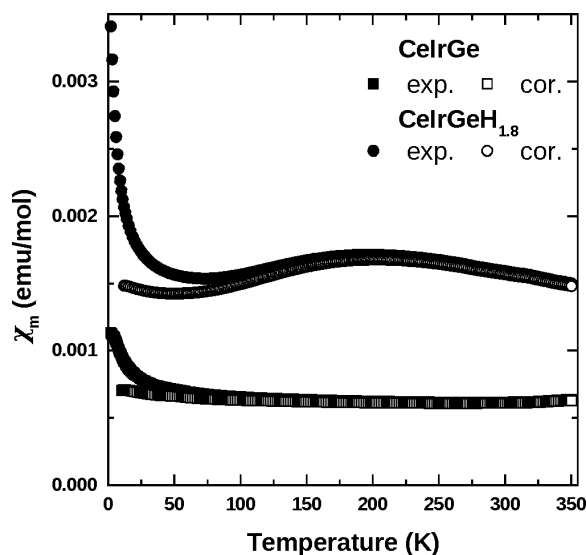
Fig. 5. Temperature dependence of the magnetic susceptibility \chi_m , measured with an applied field of 4 T, for the ternary germanide CeIrGe and its hydride. The open symbols show the corrected susceptibility [\chi_m - nC/T] (see text).
