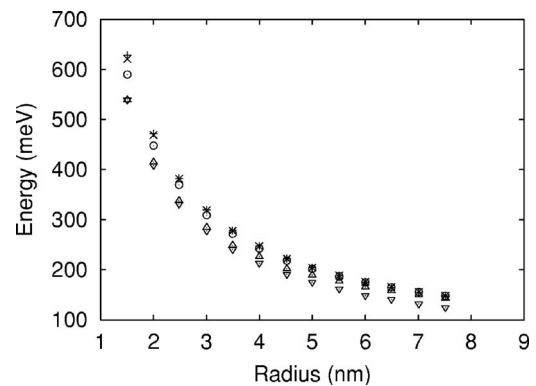
FIG. 4. Ionization energy versus the radius R for a P impurity located at different distances r=0 (+), r=0.25R ( \times ), r=0.5R ( \circ ), r=0.75R ( \triangle ) from the axis of a free-standing SiNW ( \epsilon_{\text{out}}=1 ). The symbols \nabla correspond to an impurity located at a fixed distance (0.68 Å) from the surface.
