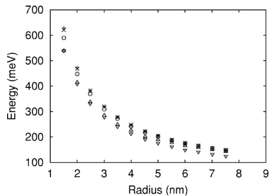
FIG. 4. Ionization energy versus the radius R for a P impurity located at different distances r=0 (+), r=0.25R ( \times ), r=0.5R ( \odot ), r=0.75R ( \triangle ) from the axis of a free-standing SiNW ( \epsilon_{\text{out}}=1 ). The symbols \nabla correspond to an impurity located at a fixed distance (0.68 Å) from the surface.
