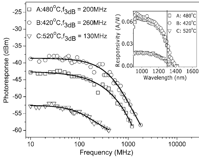
FIG. 3. Photoreponse of GaAs/GaAsSbN/GaAs photodiodes with GaAsSbN i layer grown at different temperatures measured with 1.3 \mu\text{m} laser excitation under -1 V reverse bias. (The line serves as a guide for the eyes.) Inset: dc photoreponse spectra taken under the same reverse bias.
