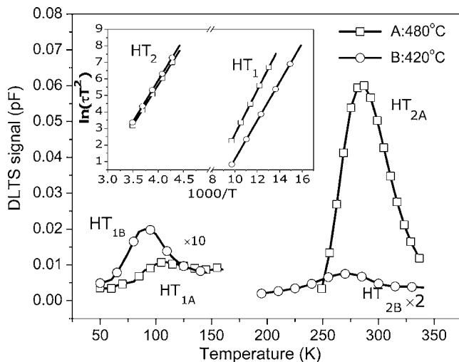
FIG. 6. DLTS spectra of photodiodes obtained using filling pulse of -0.01 V, pulse duration of 40 ms, and period width of 2 ms. Reverse bias are -2 and -4 V for samples A and B, respectively. Activation energy and hole capture cross sections were determined from the Arrhenius plots shown in the inset.
