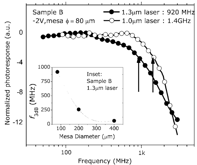
FIG. 4. Photoreponse of sample B: GaAs/GaAsSbN/GaAs photodiodes ( 80\ \mu\text{m} mesa diameter) under laser excitations at 1.3 and 1.0 \mu\text{m} and -2 V reverse bias. Inset: Plot of 3 dB cutoff frequency vs mesa diameter. (The line serves as guide for the eyes.)
