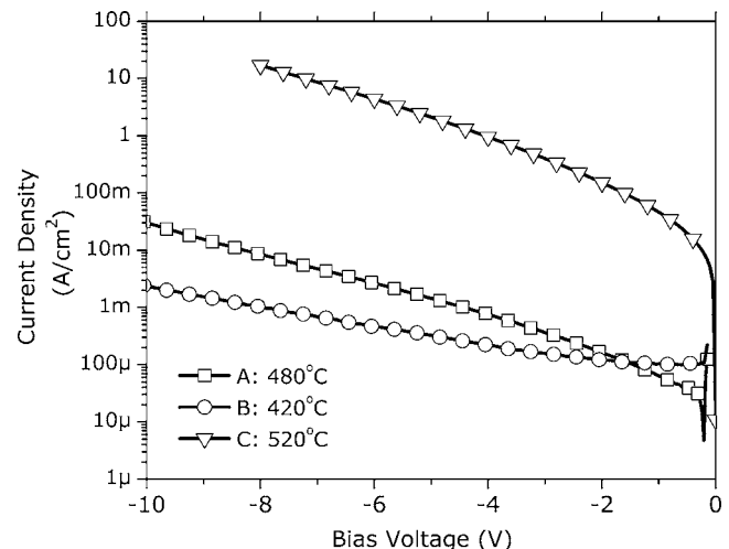
FIG. 2. Dark current characteristics of GaAs/GaAsSbN/GaAs photodiode (200 \mu\text{m} mesa diameter) with GaAsSbN i layers grown at different temperatures. Sample C with i layer grown at 520 °C is added for comparison.
