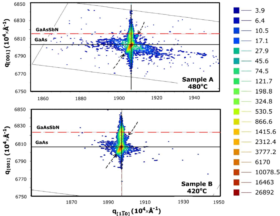
FIG. 5. (Color online) Asymmetrical reciprocal space maps of p-i-n samples in the [115] crystal orientation. The K\alpha_1 of Cu is used as the x-ray source with a wavelength of 1.54056 Å corresponding to x-ray photon energy of 8.05 keV. The dashed arrows indicate signs of local concentration fluctuations, while the diffused scattering suggests the presence of point defects. The horizontal ( q_{[1\bar{1}0]} ) and vertical ( q_{[001]} ) axes are in reciprocal lattice units ( 10^4 \times \text{\AA}^{-1} ). The GaAs (black solid line) and GaAsSbN (dashed red line) peaks are located on one vertical line, indicating closely lattice-matched condition.
