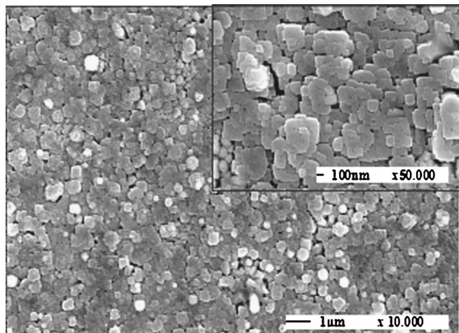
FIG. 2. Typical morphology observed by scanning electron microscopy for KTN films grown on MgO,—: 1 \mu\text{m} , inset—100 nm.
