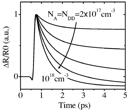
FIG. 9. Calculated transient reflectivity curves for an injection pulse of 7 \times 10^{17} \text{ cm}^{-3} electron-hole pairs and various values of N_{\text{DD}}=N_{\text{A}} (ranging from 2 \times 10^{17} to 10^{18} \text{ cm}^{-3} ).
