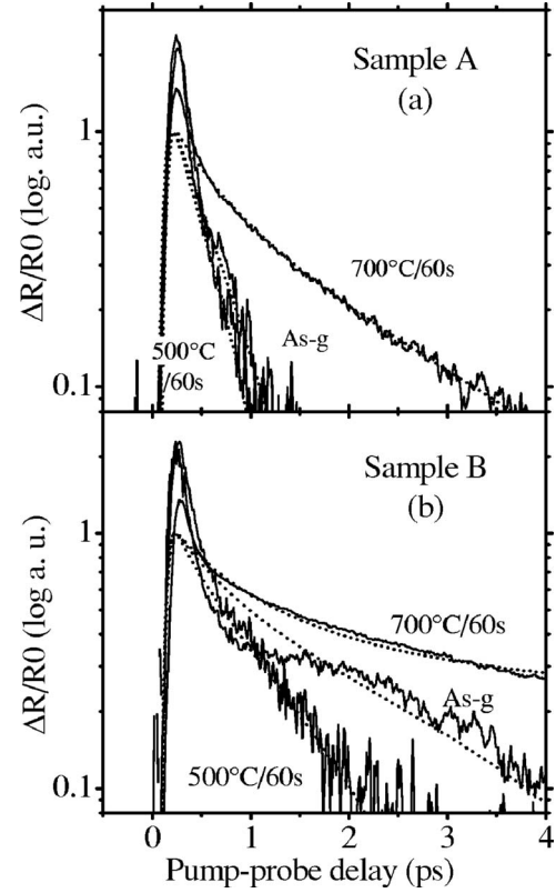
FIG. 2. Transient reflectivity signals (log scale) for sample A (top) and sample B (bottom) as-grown and annealed 60 s for 500 and 700 °C (solid lines) and their respective modeling (dotted lines).
