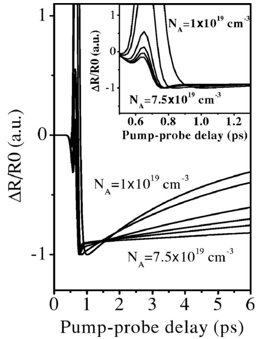
FIG. 10. Calculated transient reflectivity curves for an injection pulse of 7 \times 10^{17} \text{ cm}^{-3} and various values of N_{\text{A}} (1, 2.5, 5, 6, 6.5, and 7.5 \times 10^{19} \text{ cm}^{-3} , with fixed N_{\text{DD}}=7.5 \times 10^{19} \text{ cm}^{-3} ). Inset: zoom of the 0.5–1.2 ps region.
