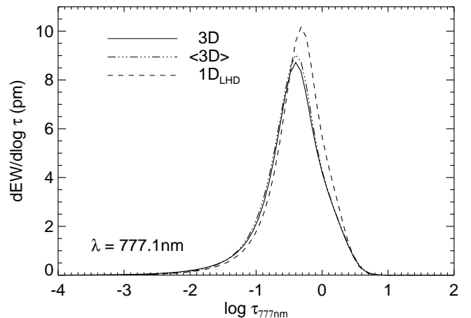
Fig. 2. The equivalent width contribution function, dEW/d\log \tau , for the 777.1 nm line at disc-centre, calculated from the 3D model (solid line), the \langle 3D \rangle model (triple dot-dashed), and the 1D LHD model (dashed). Following Magain (1986), the contribution function is defined such that integration over \log \tau_{\lambda} gives the line equivalent width.
