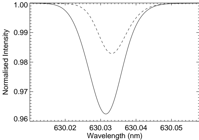
Fig. 4. The contribution of Ni I line (dashed line) with A(\text{Ni})=6.25 is compared to the combined [O I]+Ni I blend (solid line) for disc-centre according to the Linfor3D computation with A(\text{O})=8.66 .
