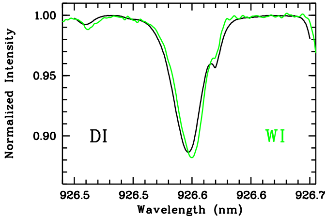
Fig. 11. The observed Delbouille (DI) and Wallace (WI) disc-centre intensity spectra of the O I 926 nm line.
