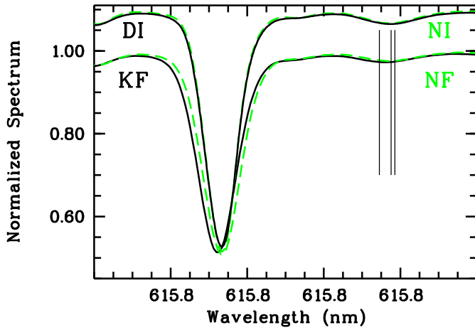
Fig. 7. The O I 615 nm Mult. 10 lines in the four observed spectra used in this work. Symbols are as in Fig. 3. The three vertical lines indicate the laboratory wavelength of the lines.
