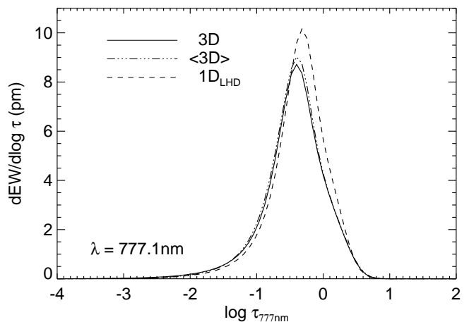
Fig. 2. The equivalent width contribution function, dEW/d\log \tau , for the 777.1 nm line at disc-centre, calculated from the 3D model (solid line), the \langle 3D \rangle model (triple dot-dashed), and the 1D LHD model (dashed). Following Magain (1986), the contribution function is defined such that integration over \log \tau_{\lambda} gives the line equivalent width.
