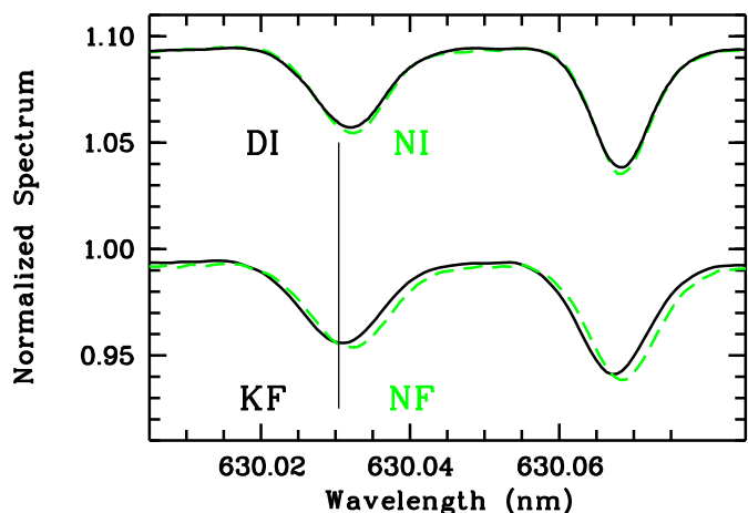
Fig. 3. The four observed spectra we used for the analysis of the [O I] 630 nm line. The Kurucz Flux spectrum, KF, and the Neckel Flux, NF, and Neckel Intensity, NI, spectra here plotted are the normalised spectra provided by Kurucz (2005a) and Neckel (1999) respectively; the Neckel Intensity, NI, is shifted up by 0.1 for clarity, while the Delbouille Intensity, DI, has been normalised and then shifted up by 0.1. The vertical line indicates the laboratory wavelength of the oxygen line. We recall that KF is corrected for gravitational redshift while NF is not, explaining the large wavelength differences between the two flux atlases
