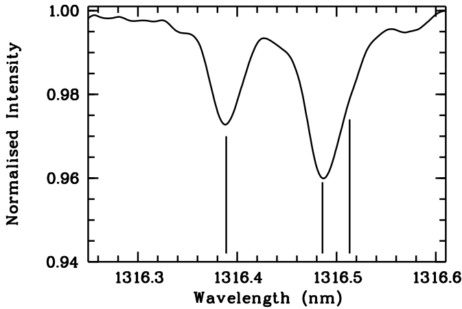
Fig. 13. The observed disc-centre intensity spectrum we have used for the analysis of the O I 1316 nm line. The vertical lines indicate the laboratory wavelengths of the three O I lines discussed in the text.
