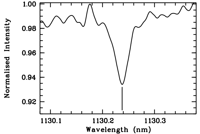
Fig. 12. The observed disc-centre intensity spectrum we have used for the O I 1130 nm line. The vertical line indicates the laboratory wavelength position of the line.
