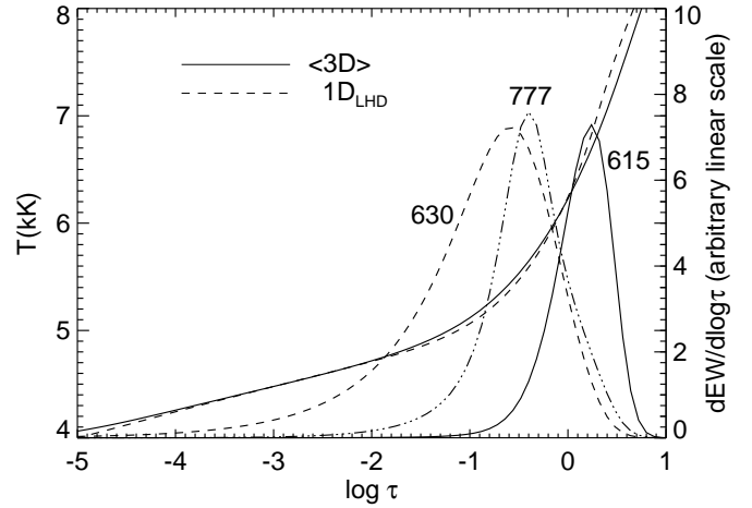
Fig. 8. The average temperature profile (left ordinate) of the 3D model (solid line) and the temperature profile of the 1D_{LHD} model (dashed) are depicted as a function of Rosseland optical depth. The EW contribution function of the disc-centre 3D synthetic spectrum (right ordinate) of the 615 nm line (solid), is compared to that of the 630 nm (dashed) and 777 nm (triple dot-dashed) lines. The contribution functions are scaled to have similar maxima and are plotted against their respective monochromatic continuum optical depths.
