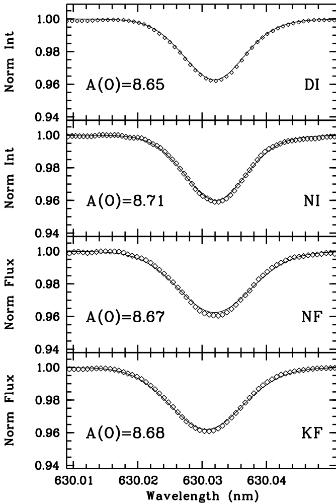
Fig. 5. The 3D fit of the [OI] 630 nm line. The observed spectra (diamonds, their size indicating the observational noise level) are over-imposed on the best fit 3D synthetic line profile (solid). From top to bottom, the spectra are: Delbouille Intensity (DI), Neckel Intensity (NI), Neckel Flux (NF), and Kurucz Flux (KF).
