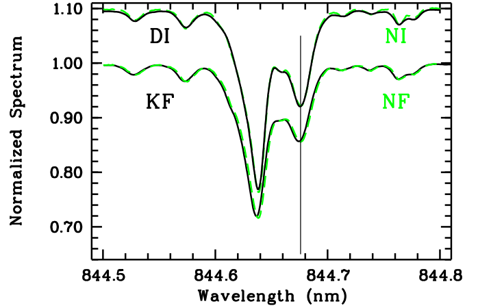
Fig. 10. The O I 844 nm line in the four observed spectra used in this work. Symbols are as for Fig. 3. The vertical line indicated the laboratory wavelength position of the line.
