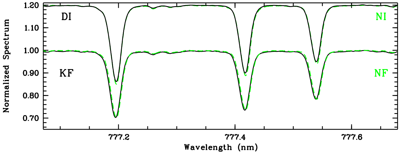
Fig. 9. The O I 777 nm triplet in the four observed spectra used in this work. Symbols are as for Fig. 3.
