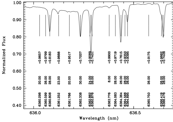
Fig. 6. The Kurucz Flux spectrum around the [OI] 636.378 nm line with the identification of the stronger lines.
