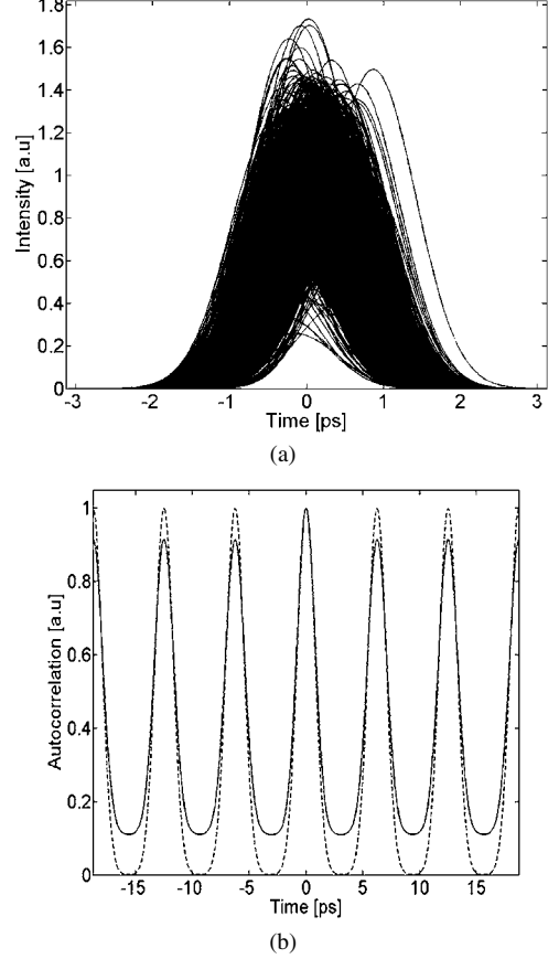
Fig. 4. (a) Eye diagram of the 160-GHz pulse train with a 4% intensity background and degraded with timing (0.2 ps) and amplitude (20%) jitters. (b) Autocorrelation function of the initial (dashed line) and degraded pulse train.
