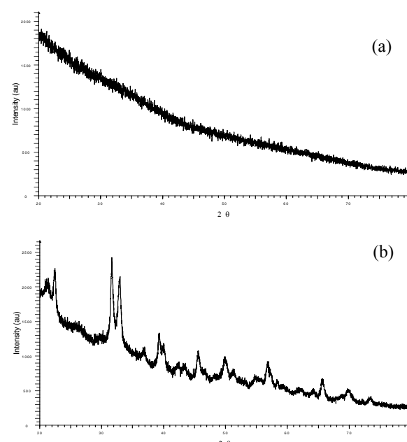
Fig.1: XRD patterns of \text{Yb:Sc}_2\text{O}_3 precursor powders (a) amorphous precipitates, (b) crystallized precipitates
