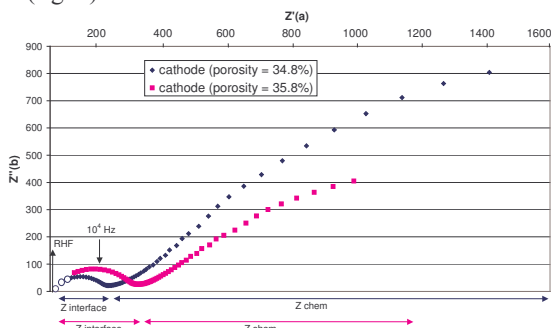
Fig.6. Nyquist diagram at 700°C of symmetrical cells \text{La}_{0.75}\text{Sr}_{0.25}\text{Mn}_{0.8}\text{Co}_{0.2}\text{O}_{3-\delta} / \text{La}_9\text{Sr}_1(\text{SiO}_4)_6\text{O}_{2.5} / \text{La}_{0.75}\text{Sr}_{0.25}\text{Mn}_{0.8}\text{Co}_{0.2}\text{O}_{3-\delta} sintered at 1400°C-2h.
