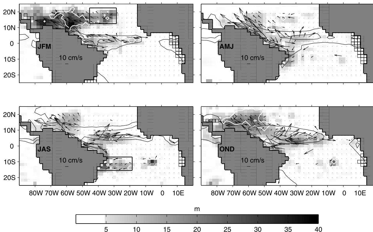
Figure 4. Grey scale gives easonal BL thickness in the tropical Atlantic basin. Grid points with no data during at least 1 month of the season are shown contoured in black. Arrows denote drifter-derived seasonal near-surface currents from Lumpkin and Garraffo [2005]. For clarity, the currents have been smoothed using a three-point hanning window over both dimensions, and only one vector out of three is shown, and only at areas where the BL is thicker than 5 m. Black contours are 4 mm/d and 8 mm/d precipitation contours from the Xie and Arkin [1997] data set. White contours are subsurface temperature maximum greater than 0.3^{\circ}\text{C} over the season (see de Boyer Montégut et al. [2007a] for details). The four panels represent an average over the four seasons as in Figure 1. The boxes highlight BL areas studied in section 6 and also shown in Figure 6.
