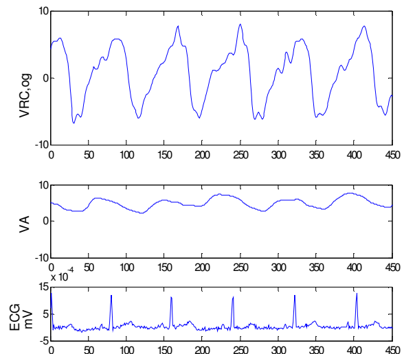
Fig. 2. V_{RC,og} , V_A (in arbitrary units) and electrocardiogram signals obtained during open glottis apnea vs. points index for subject 3. Values on the first and second y-axis are the real values*1000.
