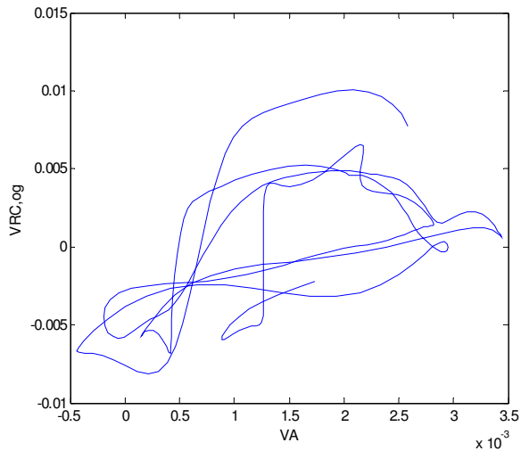
Fig. 5. VRC_{og} vs. V_A from signals of subject 3 during an open glottis apnea.
