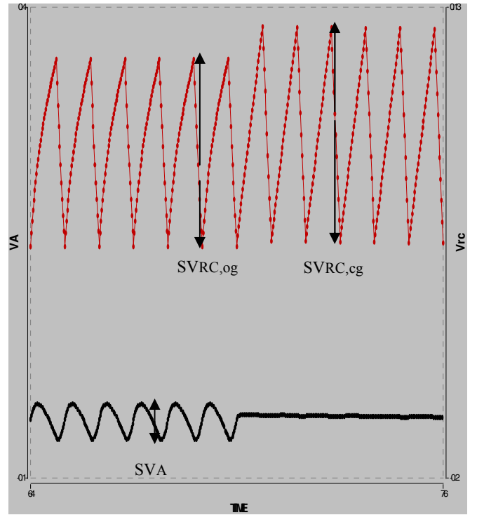
Fig. 3. Simulation of an apnea with open glottis (6 cardiac cycles) followed by apnea with closed glottis (6 cardiac cycles). Curve at the top represents VRC (L) vs time and at the bottom VA (L) vs time. SVRC,cg is higher than SVRC,og
