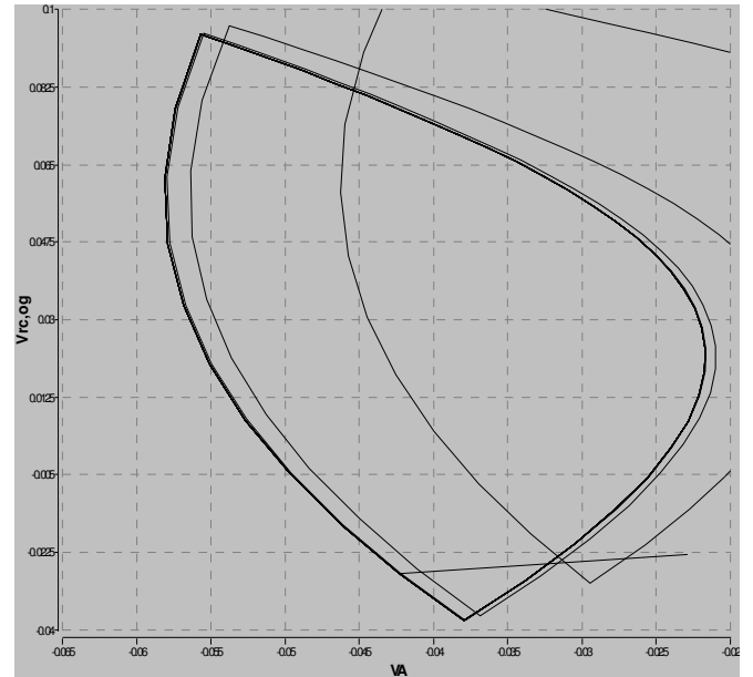
Fig. 4. VRC,og vs. VA as predicted by model.
