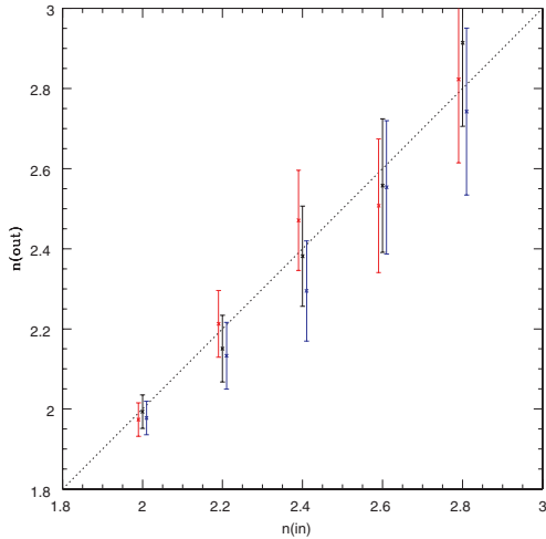
Figure 1. Results for a single ring configuration. The ring is located 100 arcsec from the cluster centre. The deformations are generated using a power-law profile whose slope is n_{\text{IN}} reported on the horizontal axis. Using the constraints provided by the rings, we estimate this slope n_{\text{OUT}} which is reported on the vertical axis. The black points with errorbars correspond to a sample of single ring around a circular galaxy, the red points to a radial configuration and the blue points to an orthoradial configuration. The black dashed line denotes the equality.
