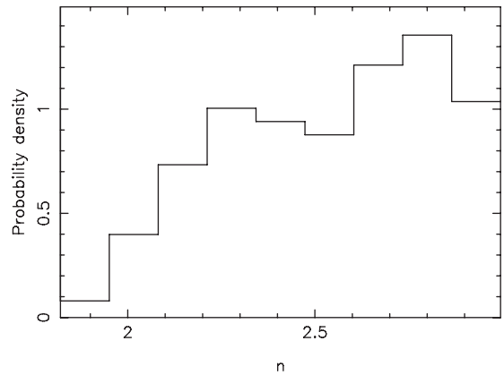
Figure 2. Top panel: dependence of the accuracy of the method with respect to the distance between ring and cluster centre R (ring). In red, the input slope is n = 2.6 , whereas in blue the input slope is n = 2.2 . Bottom panel: histogram of the probability density of n values for the point 250 arcsec and n = 2.6 taken from the top figure.
