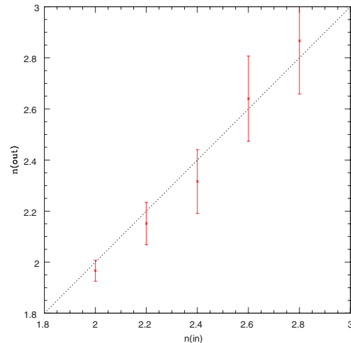
Figure 4. Results for a three ring configuration similar to Abell 1689. The rings are located 100 arcsec from the cluster centre and surround the main clump. The deformations are generated using a power-law profile whose slope is n_{\text{IN}} reported on the horizontal axis. Using the constraints provided by the rings, we measure the slope n_{\text{OUT}} .
