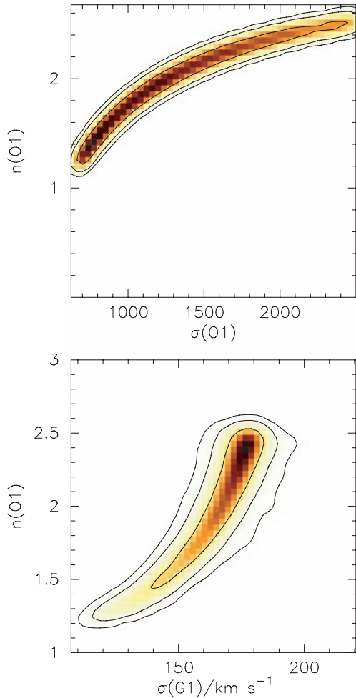
Figure 6. Degeneracies between the slope of the main central clump and dispersion of clump one and G1. The peak value found for the slope parameter is n = 2.46^{+0.06}_{-0.60} (see Table 2). These degeneracies underline the importance in obtaining the velocity dispersion of the clumps and lensed galaxies.
