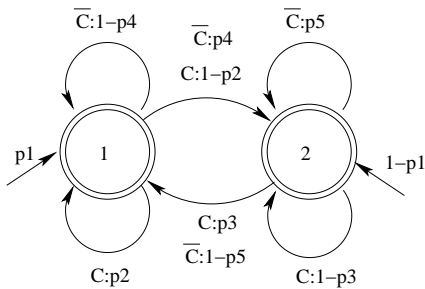
Figure 4: Probabilistic multi-strategies two-states automaton
