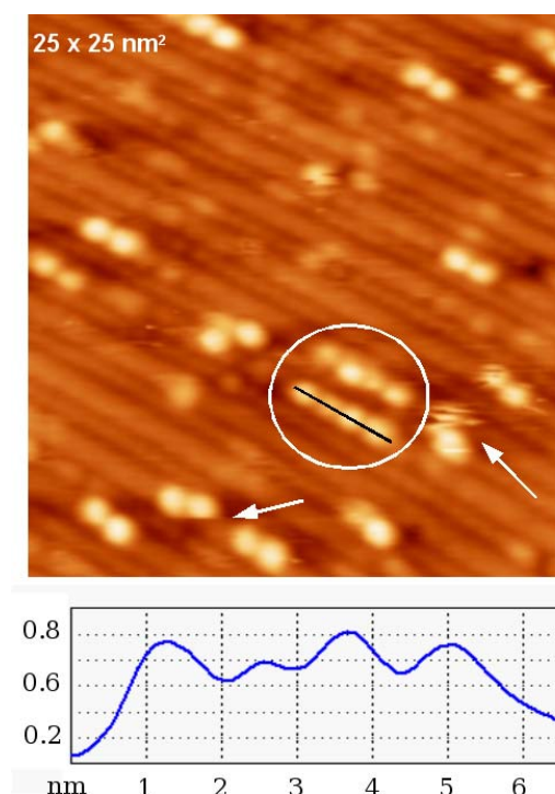
Figure 3. STM observation of the DETB subunits on SmSi(111)-8x2 interface at low coverage regime (Vs = +2.3 V, It = 0.02 nA) (top) and profile of the molecular line (down). The Sm lines are also observed on the substrate.
