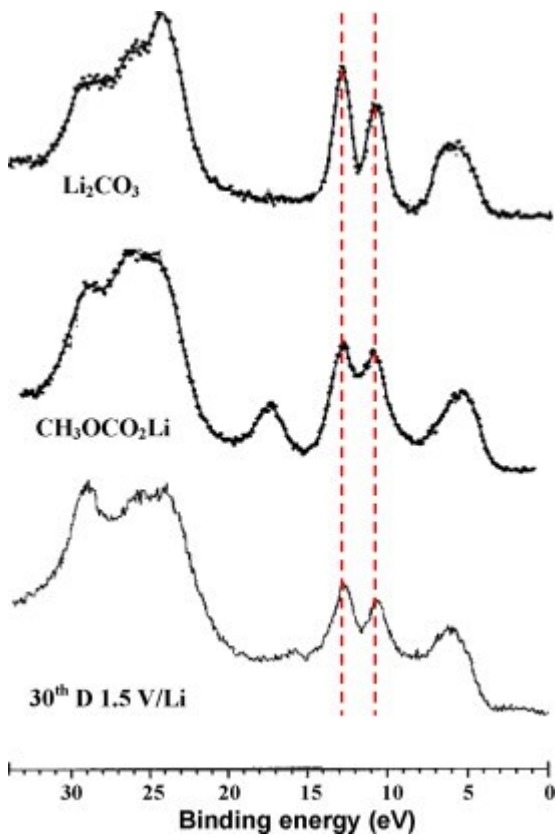
Fig. 7. XPS valence bands of Li 2 CO 3 and CH 3 CO 2 OLi as references, and for V 2 O 5 thin film at the end of the 30th discharge (V = 1.5 V/Li).
