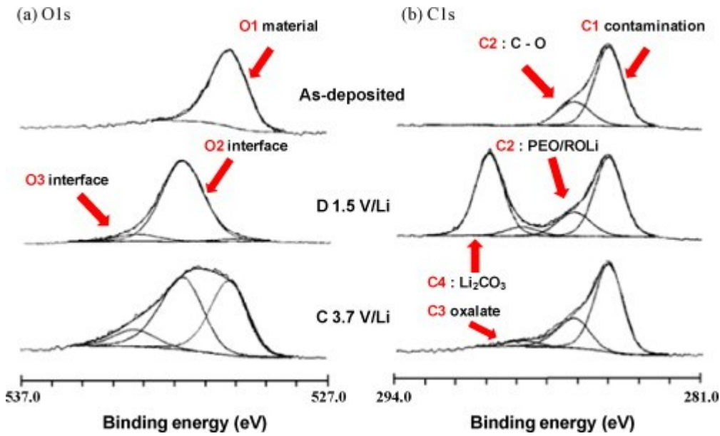
Fig. 3. XPS analyses of the O 1s (a) and C 1s (b) core peaks performed before mechanical erosion onto \text{V}_2\text{O}_5 thin films at different stages of the first cycle: the as-deposited sample, at the end of the discharge ( V = 1.5 \text{ V/Li} ) and at the end of the charge ( C = 3.7 \text{ V/Li} ).
