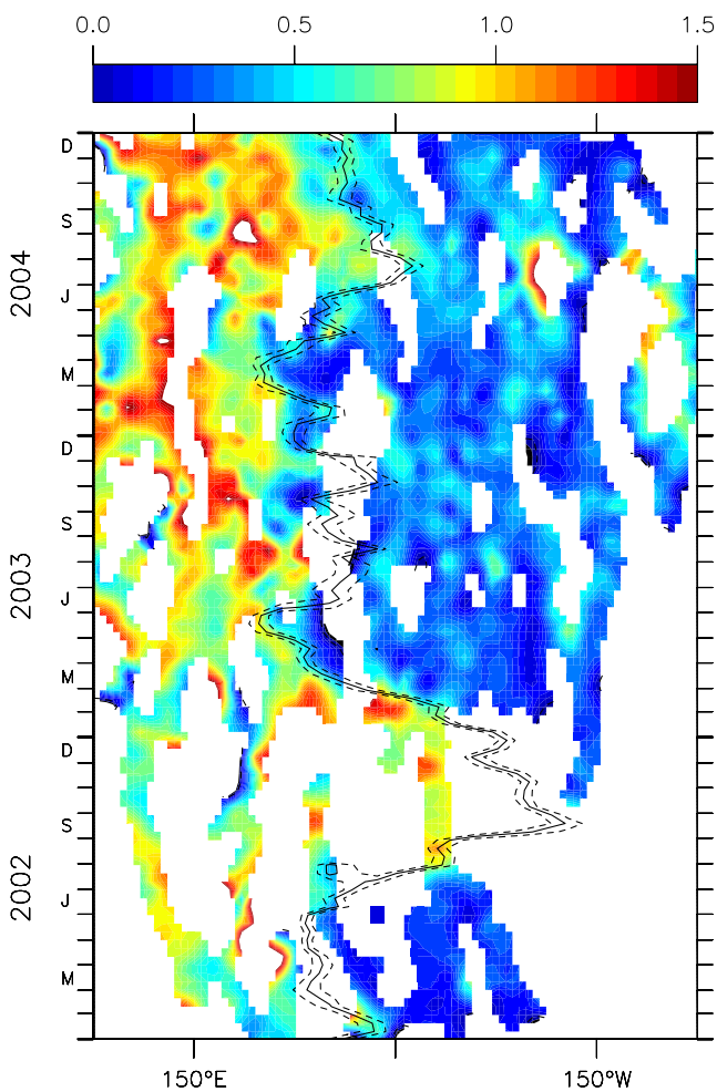
Figure 11. Longitude-time plot of the OSS (scaled by 10^{-4} \text{ s}^{-2} ) averaged for the 3^{\circ}\text{N} – 3^{\circ}\text{S} band between 140^{\circ}\text{E} and 140^{\circ}\text{W} as computed from the temperature and salinity profiles collected by the Argo autonomous floats. The solid black line represents the 34.7 isohaline and the dashed lines indicate \pm 0.2 around that value.
