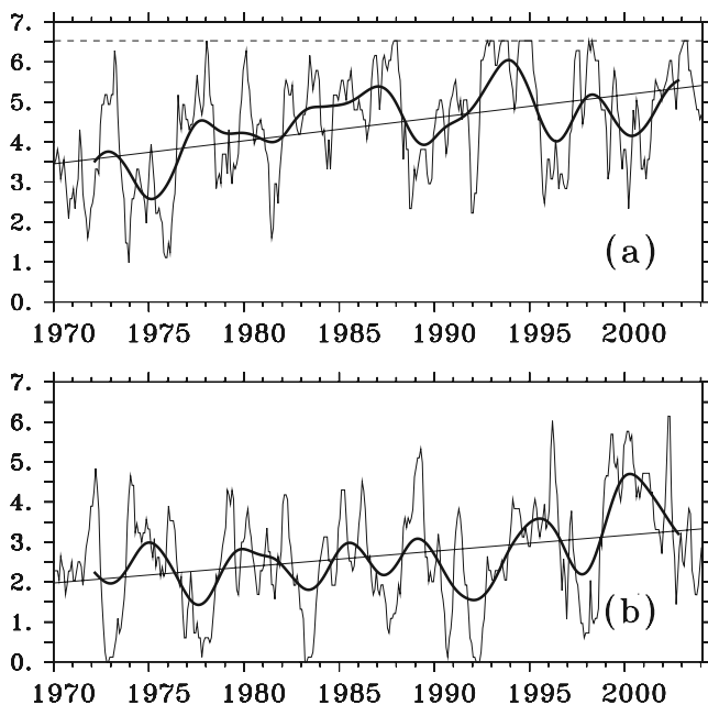
Figure 9. Monthly time series of the surface covered by (a) SSS lower than 34.8 in the 10^{\circ}\text{S} – 5^{\circ}\text{N} , 140^{\circ}\text{E} – 180^{\circ} region and (b) SSS lower than 35.0 in the 24^{\circ}\text{S} – 10^{\circ}\text{S} , 140^{\circ}\text{E} – 140^{\circ}\text{W} region. Units are 10^6 km 2 . The low-frequency curves in both plots represent the 61-month Hanning filtered values used to highlight SSS changes at periods longer than the ENSO timescale. The straight lines represent the linear least squares fits of the monthly values used to quantify linear trends. The horizontal line near 6.5 units in Figure 9a denotes the maximum possible covered surface (i.e., 40^{\circ} longitude \times 15^{\circ} latitude).
