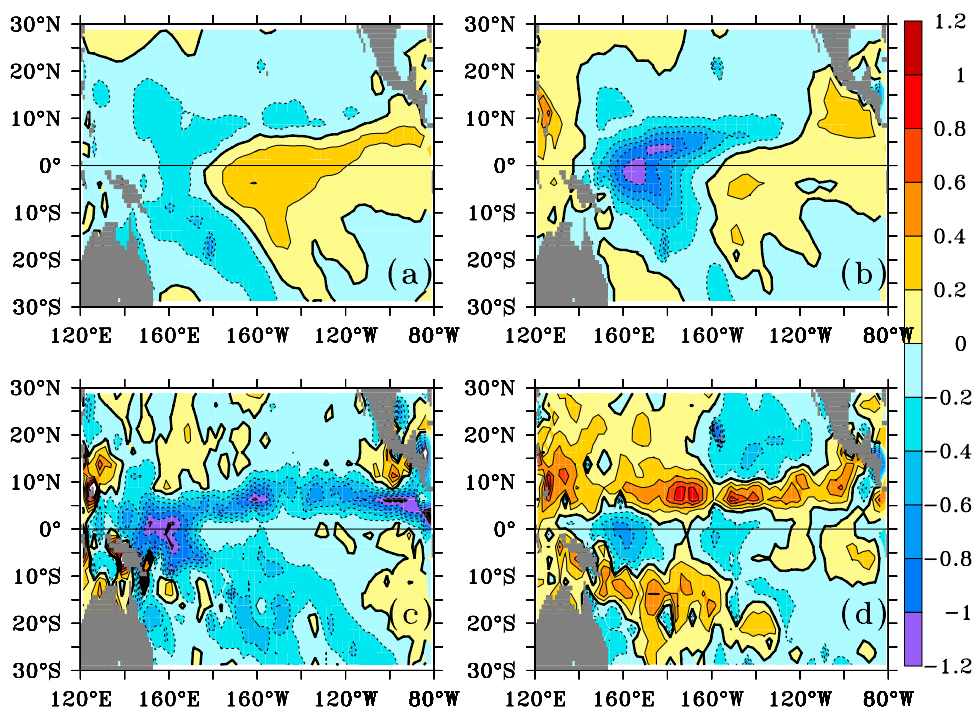
Figure 10. Comparison of precipitation trends computed from (top left) the PREC product over 1970–2003, (top right) the PREC product over 1979–2003, (bottom left) the CMAP product over 1979–2003, and (bottom right) the GPCP product over 1979–2003. See section 2 for details about the PREC, CMAP, and GPCP products. Contour intervals are 0.2, and units are m after 30 years.
