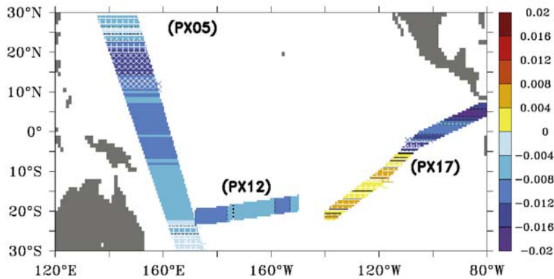
Figure 8. Linear trends in SSS along the PX05, PX12, and PX17 shipping tracks; units are psu/yr, scaled on the color bar. Lack of hatching denotes record lengths equal to or longer than 29 years; diagonal hatching is for 25–29 years; and vertical and horizontal hatching is for 19–24 years.
