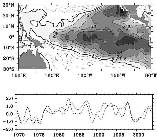
Figure 4. (top) Regression between the 1970–2003 25-month Hanning filtered SST and PDO; contour interval is 0.1, and shaded areas are positive. (bottom) Time series of 25-month Hanning filtered PDO (solid line) and reversed SOI (dashed line). Units in the top plot are defined so that the product between the contours and the PDO represents ^{\circ}\text{C} . Note that the PDO is derived as the leading EOF of monthly SST anomalies in the North Pacific Ocean, poleward of 20^{\circ}\text{N} . Positive values indicate warm phases of the PDO, with a tropical SST signal corresponding to the top plot. A schematic of the SST and wind signature of the PDO, as well as some relevant references, can be found at http://www.jisao.washington.edu/pdo/ ; see also Mantua and Hare [2002] for a PDO review.
