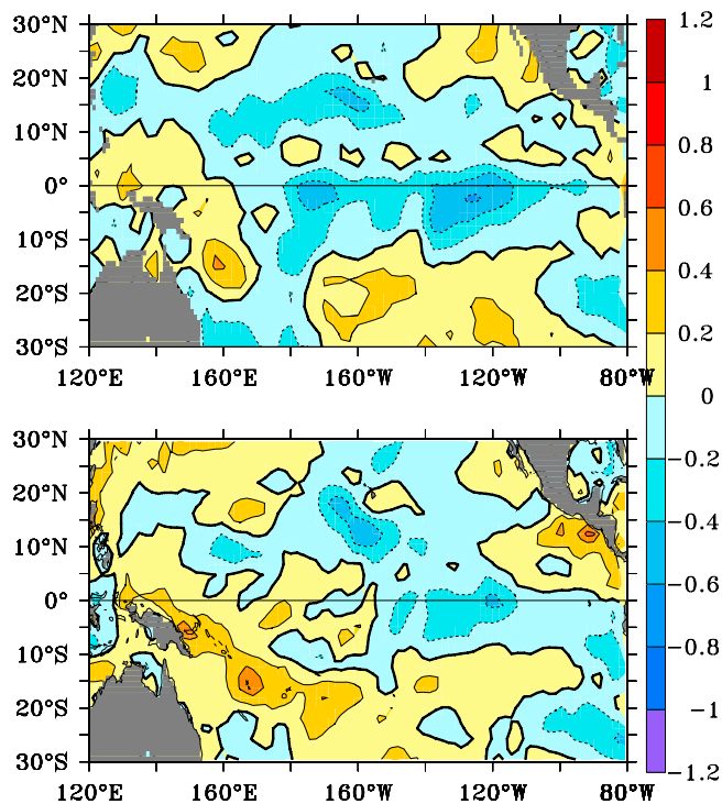
Figure 11. Comparison of evaporation trends computed from (top) the ERA40 product and (bottom) the NCEP product, both over 1970–2003. See section 2 for details about the ERA40 and NCEP products. Contour intervals are 0.2, and units are m after 30 years.
