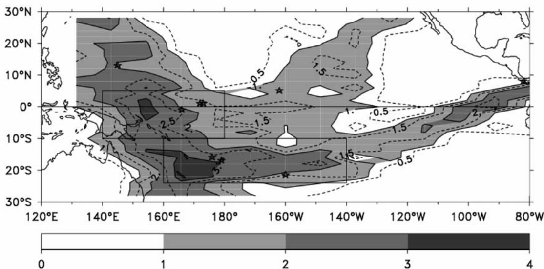
Figure 2. Lengths of SSS time series in 10^\circ longitude \times 2^\circ longitude rectangles, as expressed in decades. The two rectangles ( 10^\circ\text{S} – 5^\circ\text{N} , 140^\circ\text{E} – 180^\circ and 24^\circ\text{S} – 10^\circ\text{S} , 160^\circ\text{E} – 140^\circ\text{W} ) delimit well-sampled regions, and the nine stars represent locations with coral-derived \delta\text{O}_{18} records, as discussed in section 4.2.
