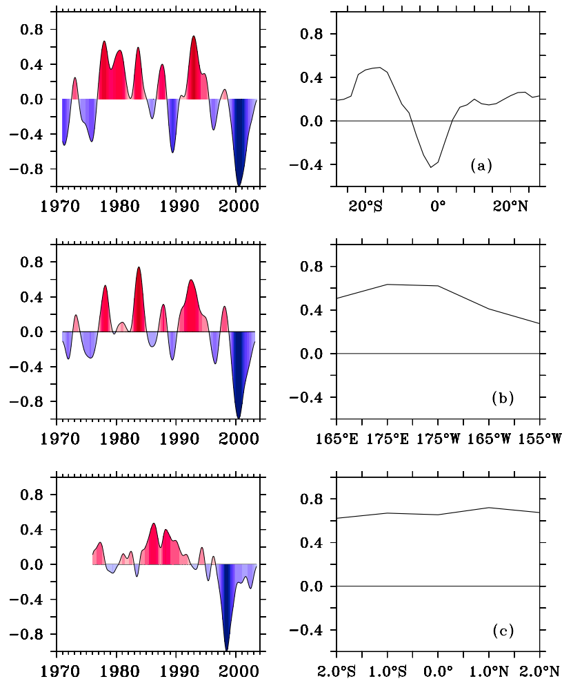
Figure 3. (left) Time functions and (right) spatial patterns of the first EOF for SSS along the (top) PX05, (middle) PX12, and (bottom) PX17 mean shipping lines. Units are defined so that the product between spatial pattern and time function represents psu. Note the different longitude and latitude scales for the spatial patterns.
