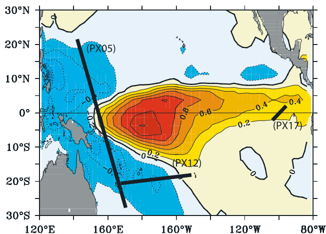
Figure 5. Regression between the 1970–2003 25-month Hanning filtered PREC precipitation product and the PDO; contour interval is 0.2, and shaded areas are positive. Units are defined so that the product between the contour values and the PDO (as shown in Figure 4) represents mm/d. Overplotted as thick black lines are the PX05, PX12, and PX17 shipping lines.
