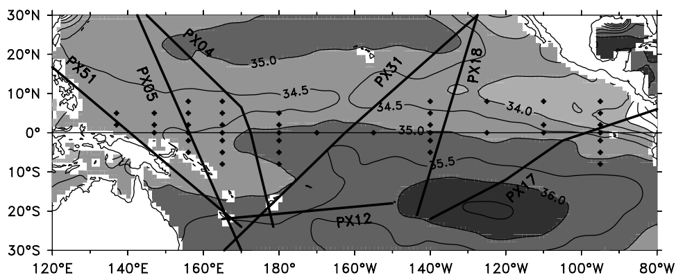
Figure 1. Long-term mean SSS in the tropical Pacific; contour interval is 0.5. Overplotted are the well-sampled shipping lines (PX51, PX05, etc.; heavy black lines) and the TAO/TRITON moorings (black dots) providing SSS observations.
