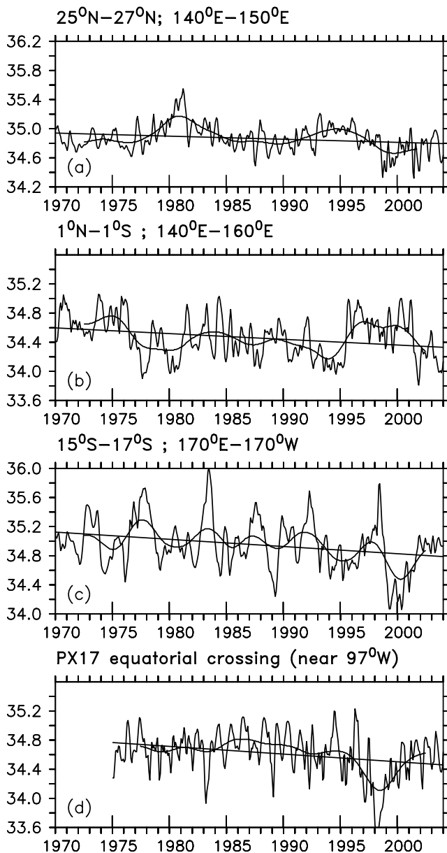
Figure 6. Time series of monthly SSS values at reported locations. The low-frequency curves represent the 61-month Hanning filtered values used to highlight SSS changes at periods longer than the ENSO timescales. The straight lines represent the linear least squares fits of the monthly values used to quantify linear trends.
