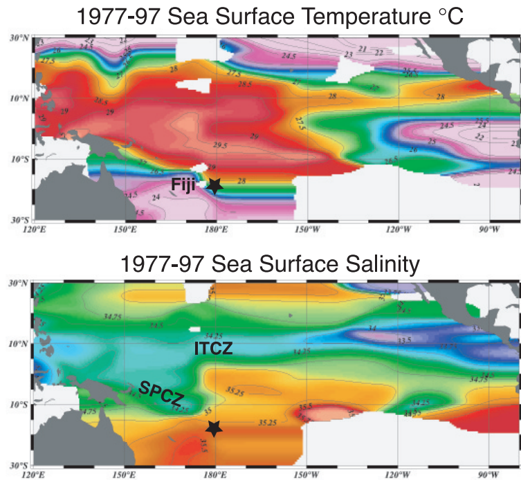
Figure 1. Annual average SST and SSS from the WOCE “Upper Ocean Thermal Programme” for the tropical Pacific Ocean during the 1977–97 period. SSS is in practical salinity units. The convergence zones ITCZ and SPCZ are indicated, underlined by low salinity.
