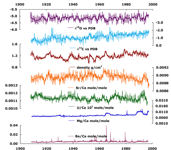
Figure 2. Monthly values of \delta^{18}\text{O} (‰ vs PDB), \delta^{13}\text{C} (‰ vs PDB), density ( \text{g}/\text{cm}^3 ), Sr/Ca (mole/mole), Mg/Ca (mole/mole), U/Ca ( 10^3 mole/mole) and Ba/Ca (mole/mole). The thicker curves denote the 25-month Hanning filtered signals.
