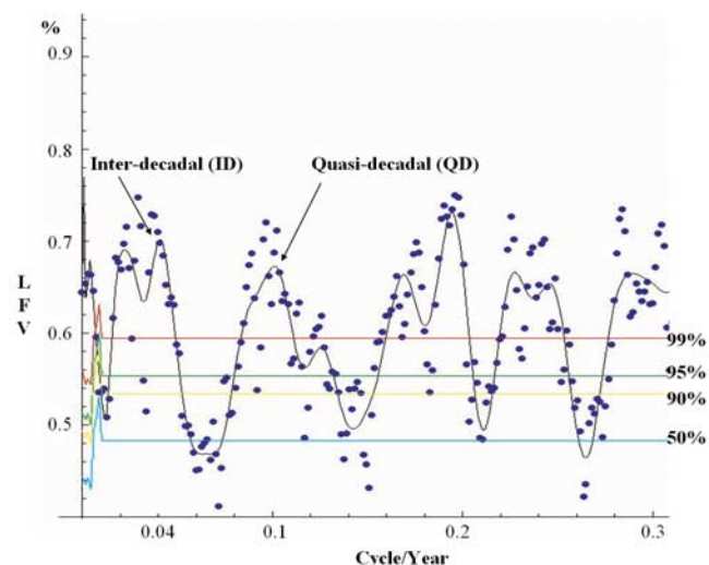
Figure 1. Local Fractional Variance (LFV) for joint SSTA-SLPA analysis, using MTM/SVD. Blue dots are joint LFV values prior to smoothing. Thin black line is obtained from polynomial smoothing. Peaks for Inter-decadal and Quasi-decadal are highlighted. Horizontal lines represent Monte Carlo significance levels. Cycle/year on abscissa.
