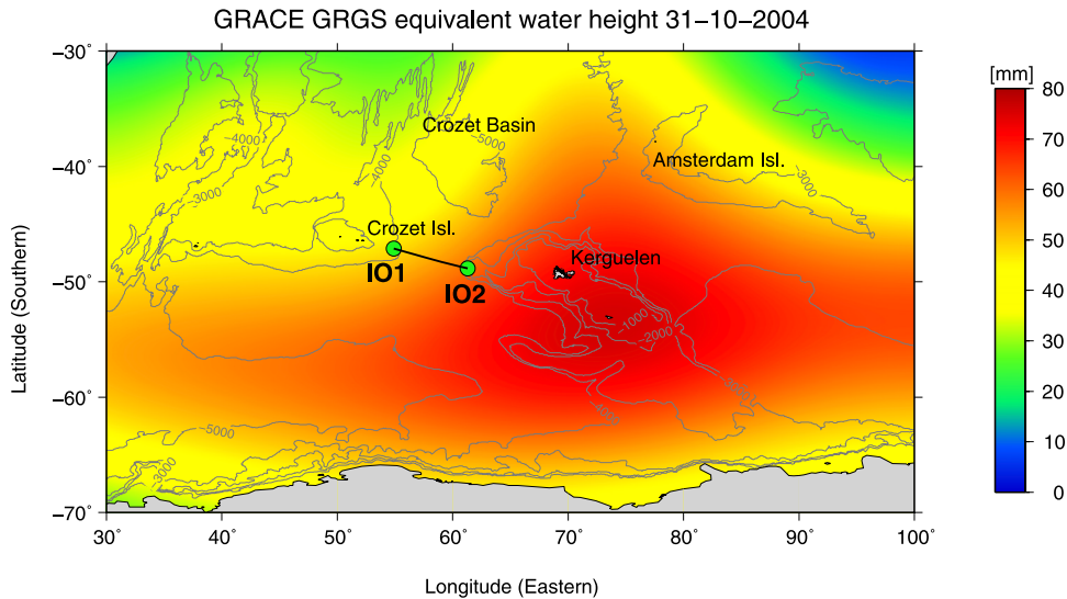
Figure 1. GRACE equivalent water height field for the solution of 31-10-2004. Note the strong anomaly at the Kerguelen plateau. Superimposed are the bathymetric contours and the positions of the BPR deployments denoted by IO1 and IO2.
