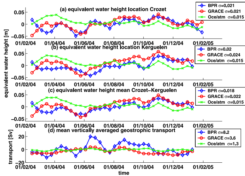
Figure 2. Equivalent water height at the BPR location (a) near Crozet, (b) near Kerguelen, (c) at the midpoint and (d) the change of the mean vertically averaged transport through the section bounded by both BPRs. Equivalent water height and geostrophic transport are given for 1) the averaged BPR data (blue diamonds), 2) GRACE (red circles) and 3) sum of barotropic ocean model (MOG2D) and ECMWF pressure fields (green crosses). The smoothing radius used is 800 km. Standard deviations are denoted by \sigma .
