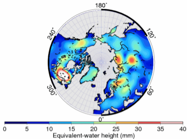
RMS --- GRACE/LaD --- 2002-2004
