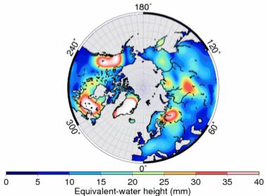
RMS --- GRACE/GLDAS --- 2002-2004
