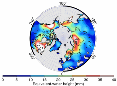
RMS --- GRACE/WGHM --- 2002-2004
