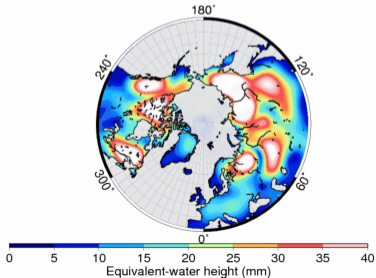
RMS --- GRACE/SSM/I --- 2002-2003
